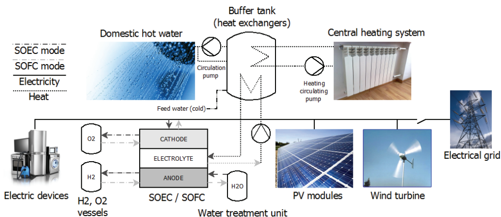
Fig. 3. Hydrogen installation scheme
