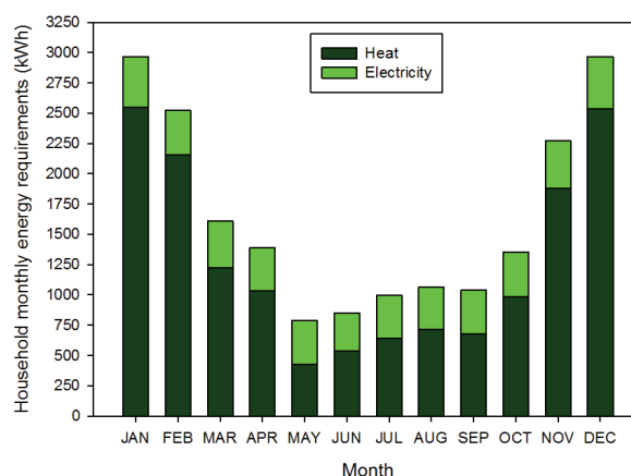
Fig. 2. Heat and electric energy requirements of the analysed household
