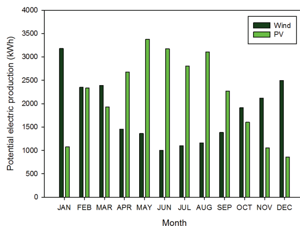
Fig. 1. Potential electric energy production from RSE installations
