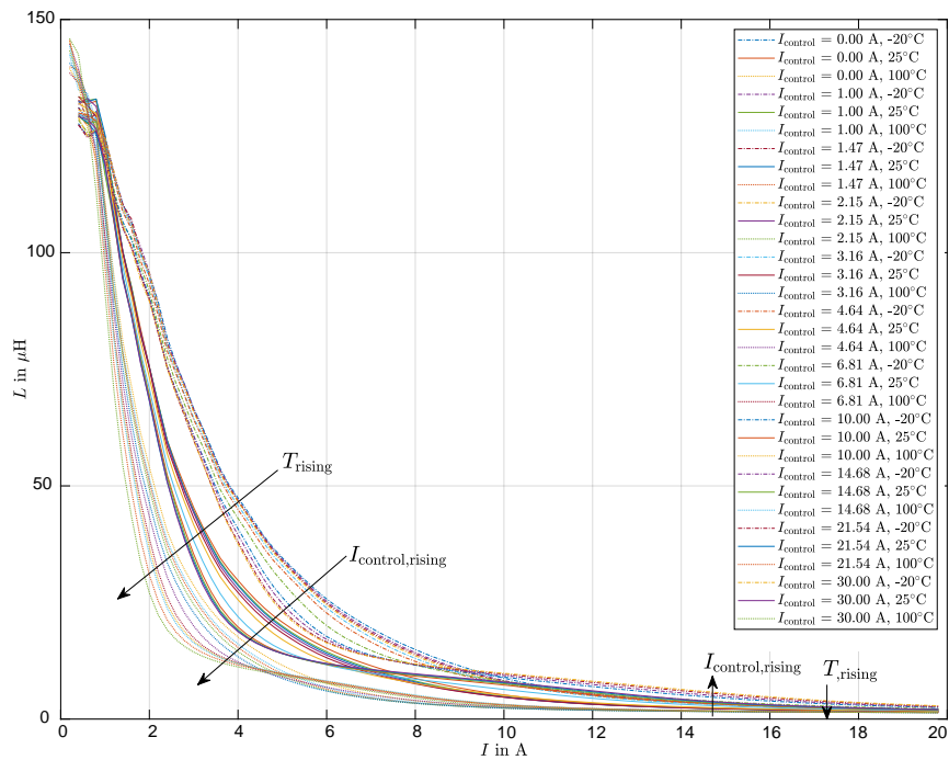
Fig. 5. Dependency of effective inductance on control current at different temperatures
