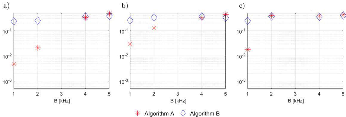
Fig. 16. The BER of the simulated transmission using DSSS signals constructed of Kasami codes of rank 6 in NOF1 (a), NCS1 (b), and BCH1 (c) Watermark channel.
