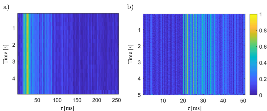
Fig. 18. Modules of TVIRs measured in the model pool using signals of bandwidth equal to 1 kHz (a) and 5 kHz (b).
