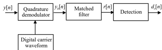
Fig. 4. Digital processing path of DSSS signal at the receiver side.
