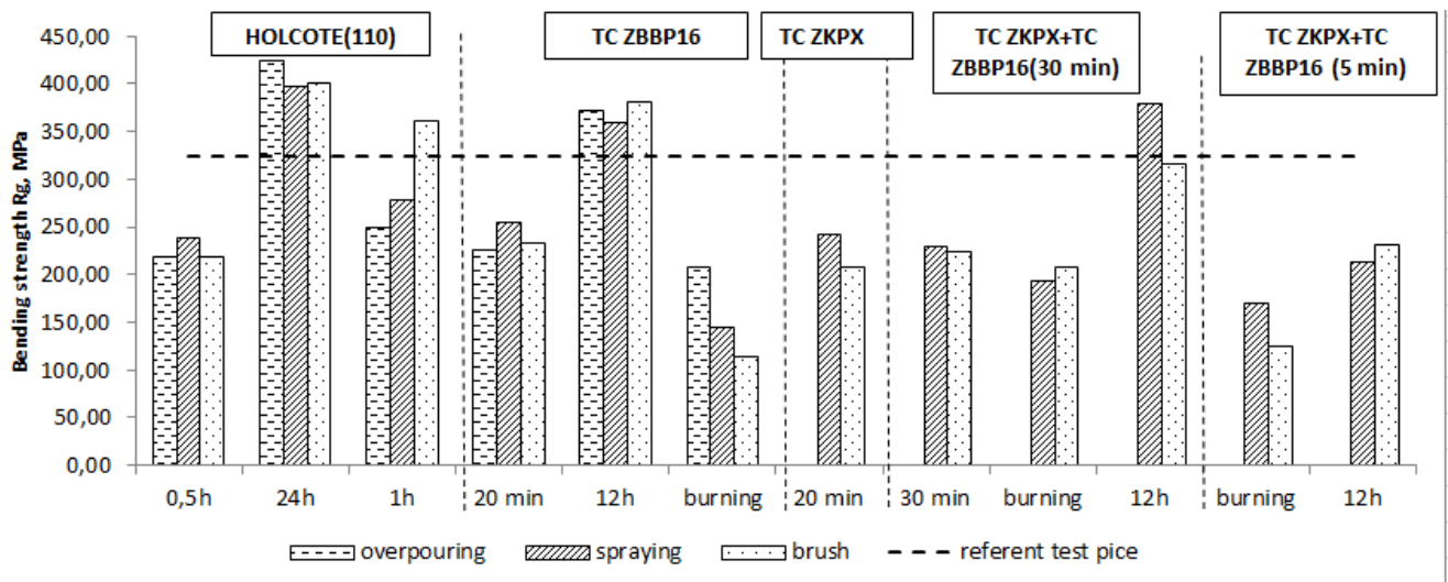
Fig. 2. Influence of different kind of coatings on bending strength of furan moulding sand
