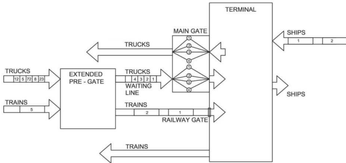
Figure 1. The scheme of the cargo flow at the container terminal, working under conditions of extended pre-gate accompanied by rail siding.
