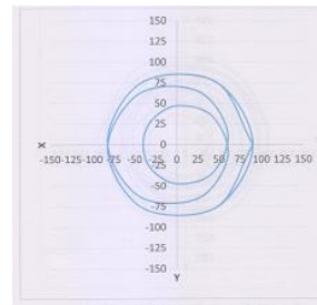
Rys. 8. Tory ruchu punktu Q dla: a) r' = 18 mm, b) r' = 9 mm, c) r' = 0 ( R = 65 mm, \omega_1 = 3\pi rad/s, \omega_2 = \pi rad/s, \omega_3 = 0,1\pi rad/s)
