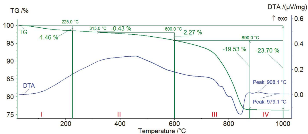
Fig. 2. Results of thermal analysis DTA/TG of waste sludge from washing dolomite aggregates
