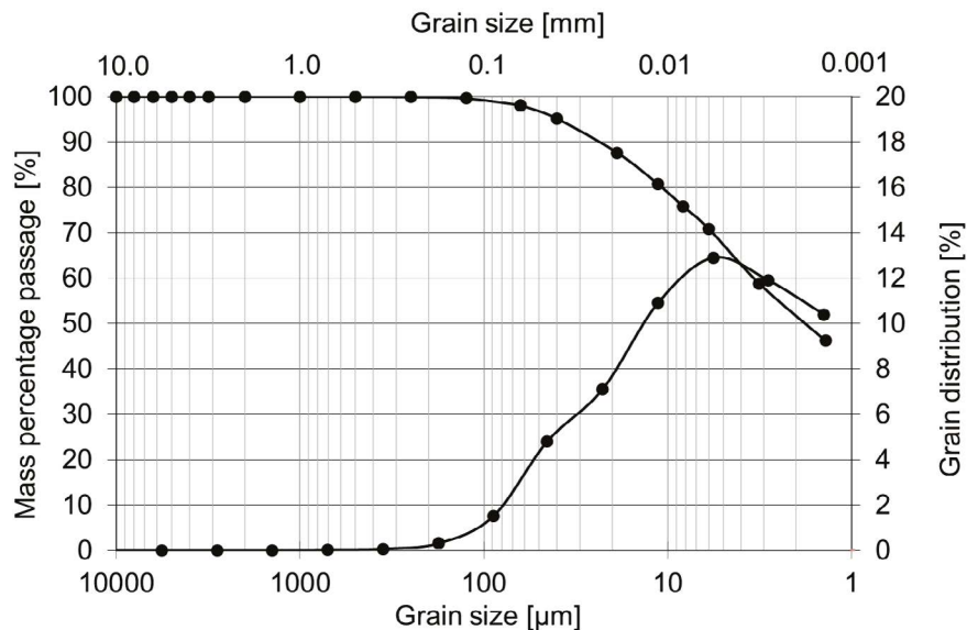
Fig. 1. Grain size of waste sludge from washing dolomite aggregates
