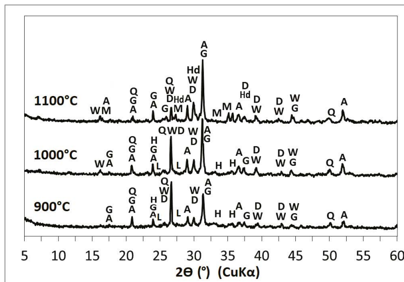
Fig. 3. XRD analysis of materials obtained from waste sludge from washing dolomite aggregates at three temperature A – akermanite, D – diopside, G – gehlenite, H – hematite, Hd – hedenbergite, M – mullite, L – leucite, Q – quartz, W – wollastonite
