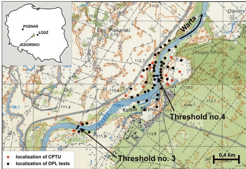
Fig. 1. Location of CPTU and DPL tests on topographic map (topographic maps of Pęcńiew and Uniejów, OPGK Poznań, 1986, modified)
