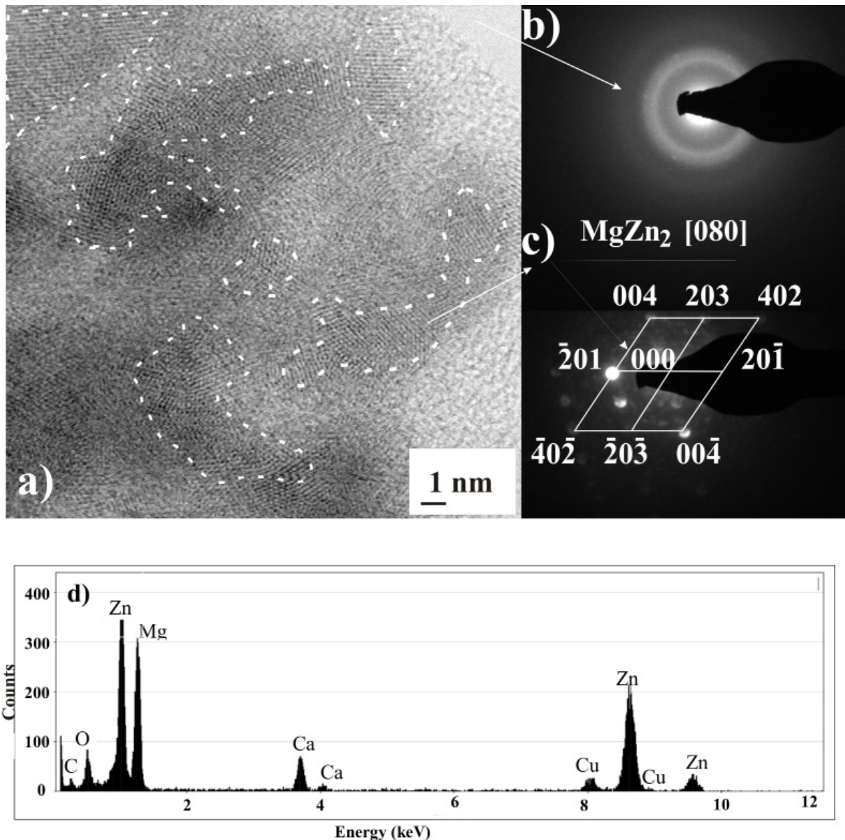
Fig. 2. Structure of the Mg_{60}Zn_{35}Ca_5 powders prepared by MA method after milling time 13 h; a) HRTEM image; b) electron diffraction from selected area marked with an arrow on Fig. a, confirm of an amorphous and c) nanocrystalline MgZn_2 phase; d) EDS spectrum
