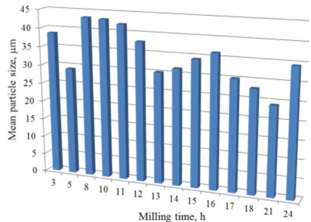
Fig. 4. Evolution of the D_{50} parameter versus milling time as derived from particle sizes distribution of the Mg_{60}Zn_{35}Ca_5 powder
