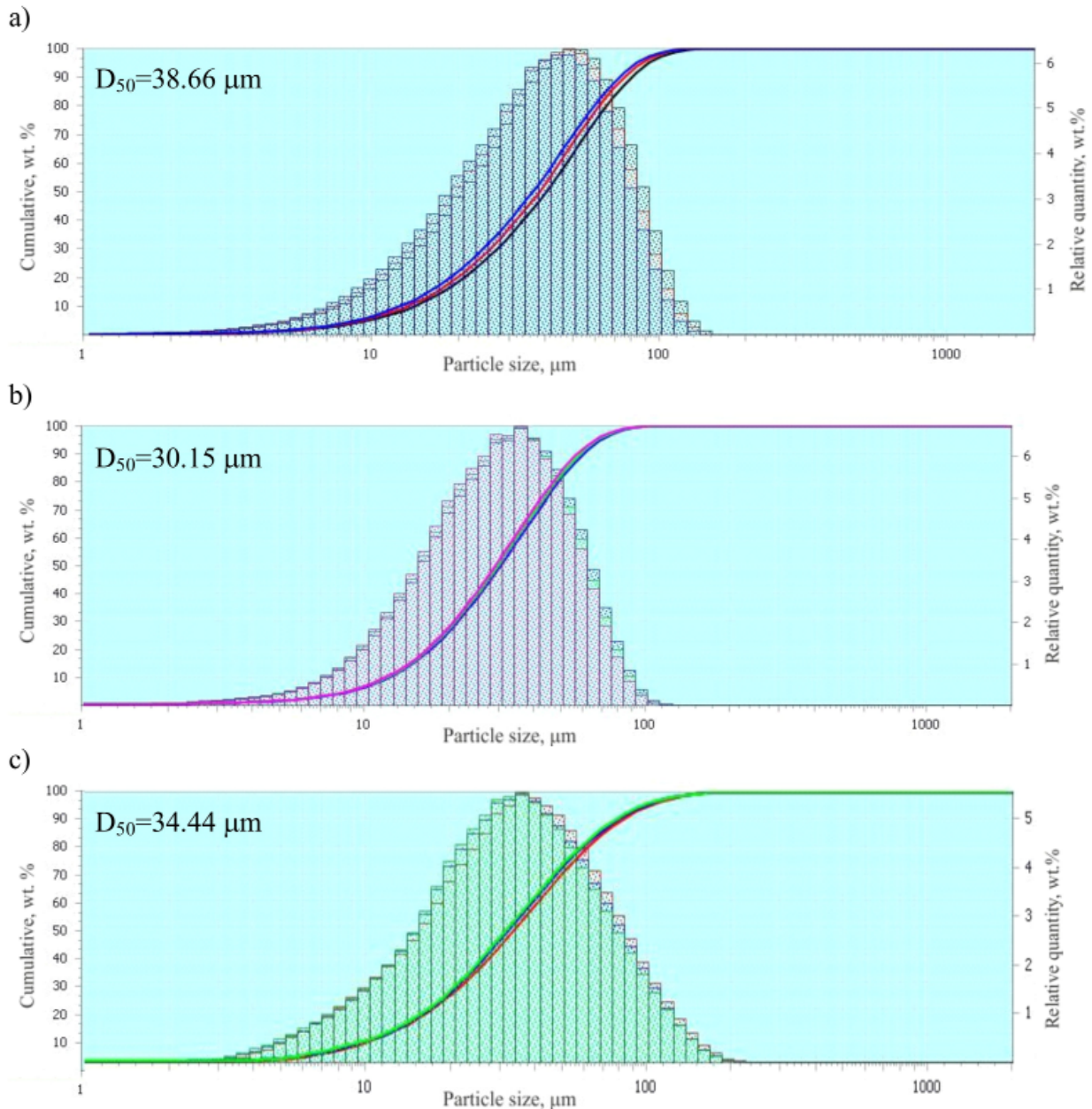
Fig. 3. Particle size distribution for the Mg_{60}Zn_{35}Ca_5 alloy milled from 3-24h: a) 3h, b) 13h, c) 24 h. For comparison reasons, the mean particle size ( D_{50} ) is given
