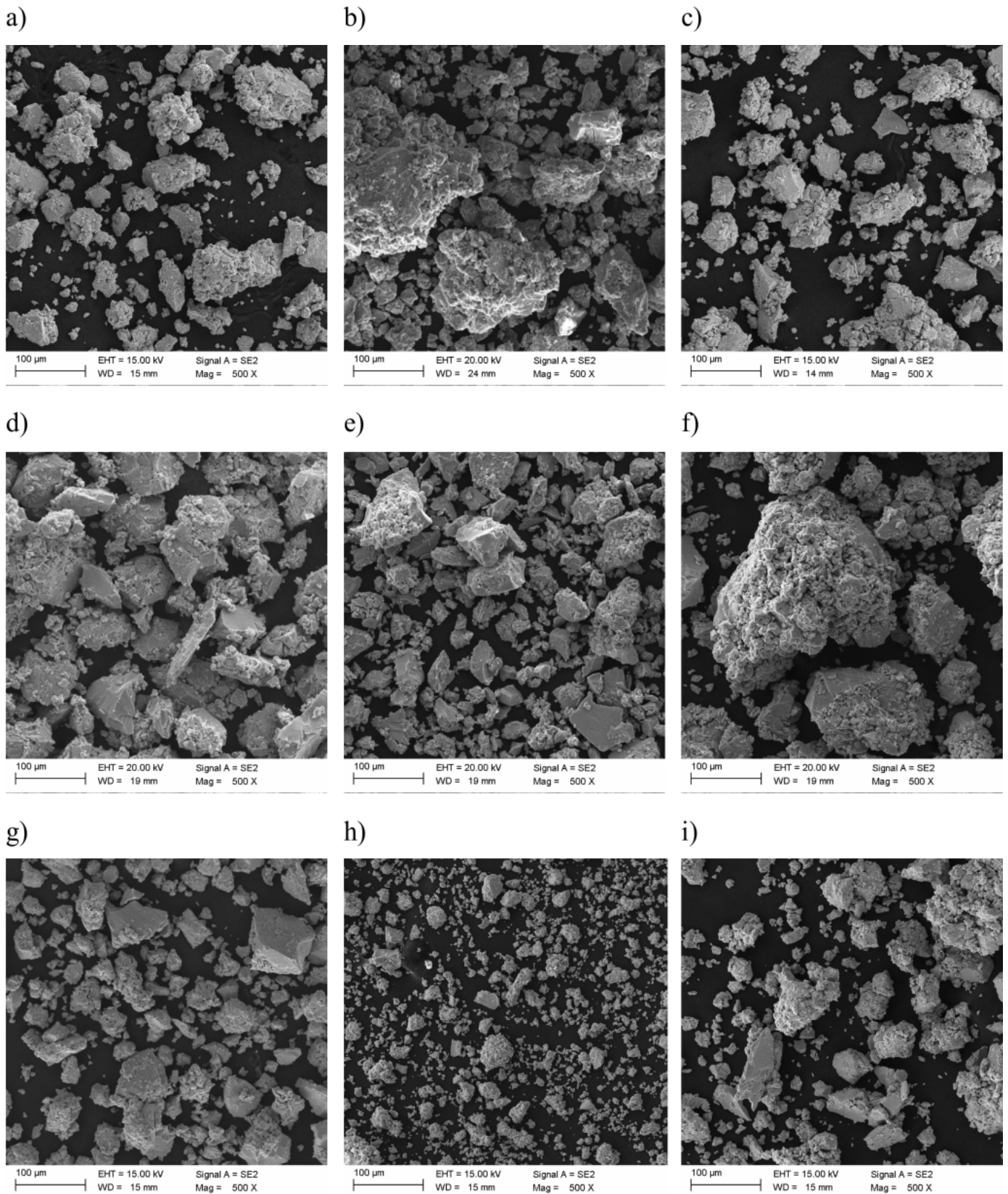
Fig. 5. The morphology of the \text{Mg}_{60}\text{Zn}_{35}\text{Ca}_5 particles after different times of milling (3-24h): a) 3h, b) 5h, c) 8h, d) 11 h, e) 13h, f) 15 h, g) 18 h, h) 21 h, i) 24 h, SEM
