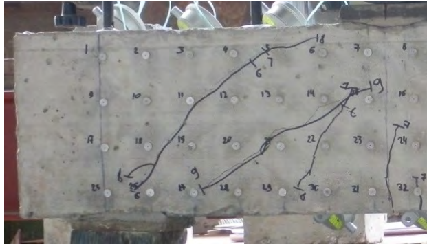
Fig. 1. Distribution of inclined cracks in the control sample
