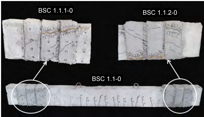
Fig. 4. The tested strengthened beam BSC 1.1-0
