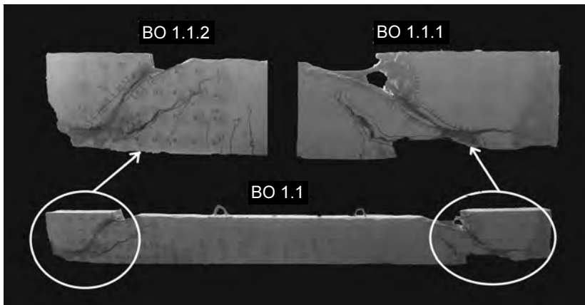
Fig. 2. The tested control beam BO-1.1
