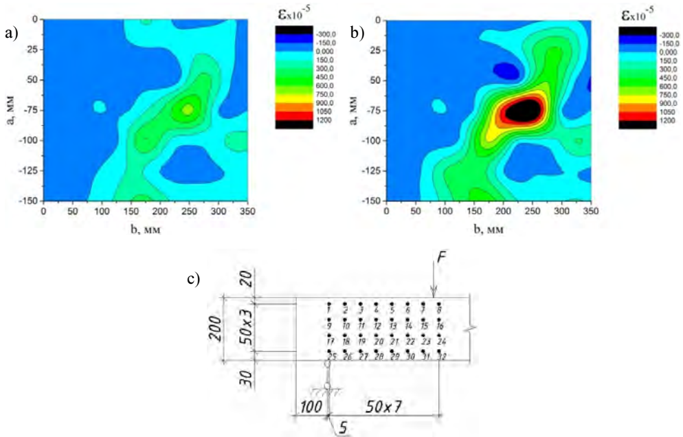
Fig. 3. The distribution of concrete deformation in the shear area for beam BO-1.1: a) the area before the opening inclined crack; b) the area before the exhaustion of ULS; c) the scheme of rappers of the comparator measurement
