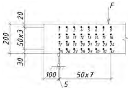
Fig. 7. The distribution of strain in the beam: area of deformation before opening inclined cracks in the beam: a) BSC 1.1-0; c) BSC 1.2-0.3; e) BSC 1.3-0.5; area of deformation before exhaustion bearing capacity for beams: b) BSC 1.1-0; d) BSC 1.2-0.3; f) BSC 1.3-0.5; g) layout rappers of the comparator
