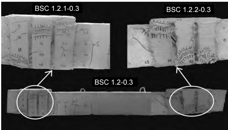
Fig. 5. The tested strengthened beam BSC 1.2-0.3
