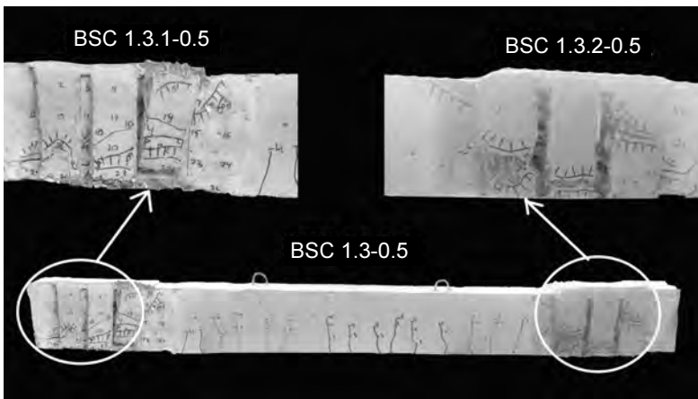
Fig. 6. The tested strengthened beam BSC 1.3-0.5
