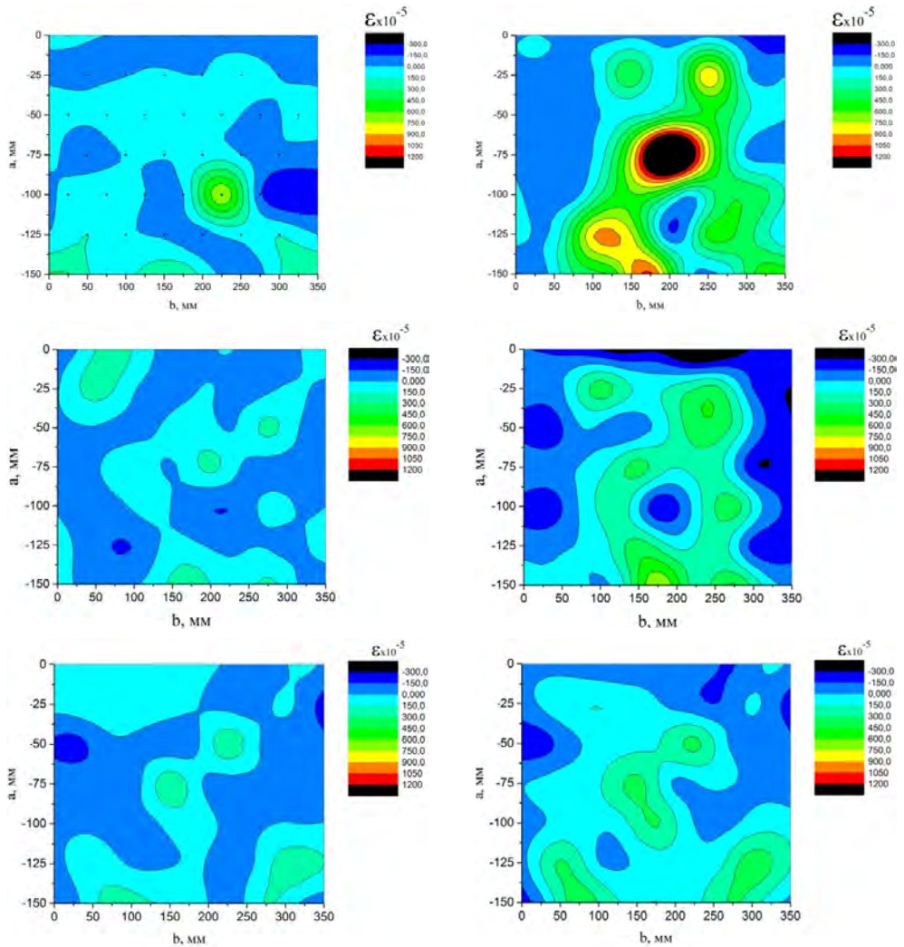
Fig. 7. The distribution of strain in the beam: area of deformation before opening inclined cracks in the beam: a) BSC 1.1-0; c) BSC 1.2-0.3; e) BSC 1.3-0.5; area of deformation before exhaustion bearing capacity for beams: b) BSC 1.1-0; d) BSC 1.2-0.3; f) BSC 1.3-0.5; g) layout rappers of the comparator
