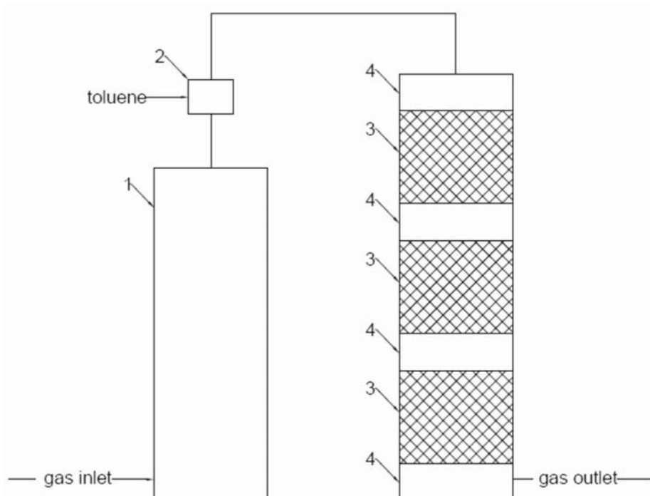
Fig. 1. Research installation scheme: 1 – column for gas pre-conditioning, 2 – mixer, 3 – filter bed, 4 – ports (Miller et al. 2019)
