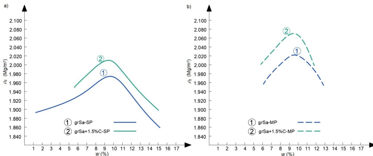
Figure 4: Compaction curves of gravelly sand and gravelly sand with 1.5% of cement addition compacted by two methods: a) SP, b) MP.
