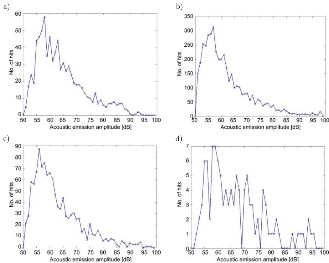
Fig. 12. Actual amplitude distribution plots: a) with inherent micro defects, b) with defect free weld, c) with weld defect, d) with HAZ failure.
