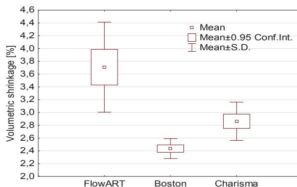
FIG. 3. Volumetric shrinkage of tested materials.
