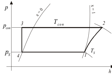
Fig. 4. Thermodynamic cycle of compressor heat pump in a Mollier graph
