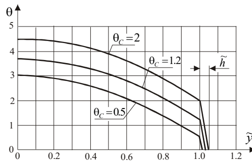
Fig. 2. Temperature distribution in a component with heat source for \tilde{q}_v = 5 and \tilde{\lambda} = 8 [1]
