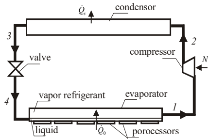
Fig. 3. Compressor heat pump schematic
