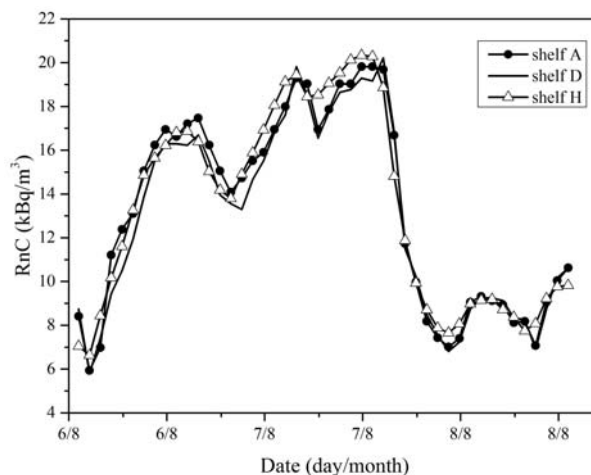
Fig. 4. Radon levels during the low-exposure test.
