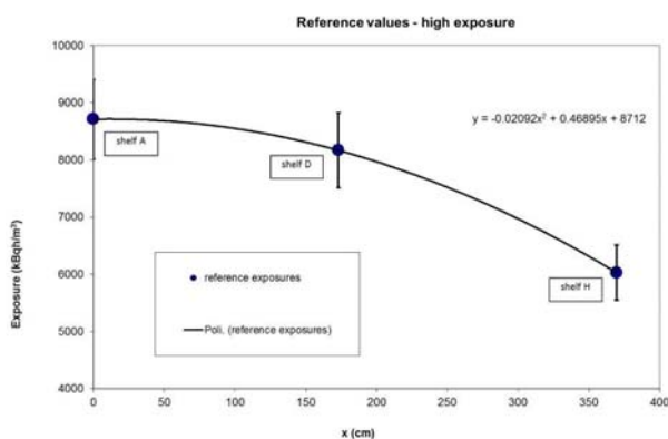
Fig. 6. High-exposure experimental reference values and the polynomial interpolation.
