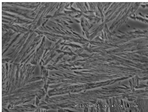
Fig. 1. An example of the microstructure of ductile iron ADI matrix
