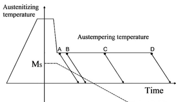
Fig. 2. Schematic representation of isothermal transformation of ductile iron [12]
