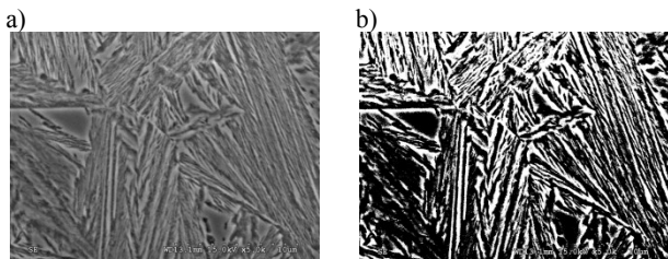
Fig. 5. a) SEM image in shades of gray, b) SEM image after the binarization process
