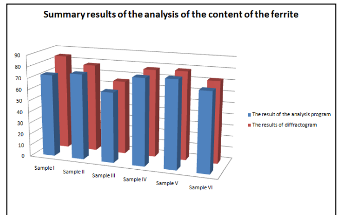
Fig. 10. Chart of the analysis of the content of Ferrite for analysis done by the program and the diffraction patterns
