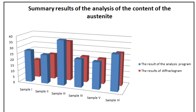
Fig. 9. Chart of the analysis of the contents of austenite for the analysis carried out by the program and the diffraction patterns
