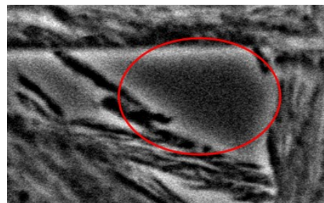
Fig. 7. Austenite block in the microstructure of ductile iron ADI
