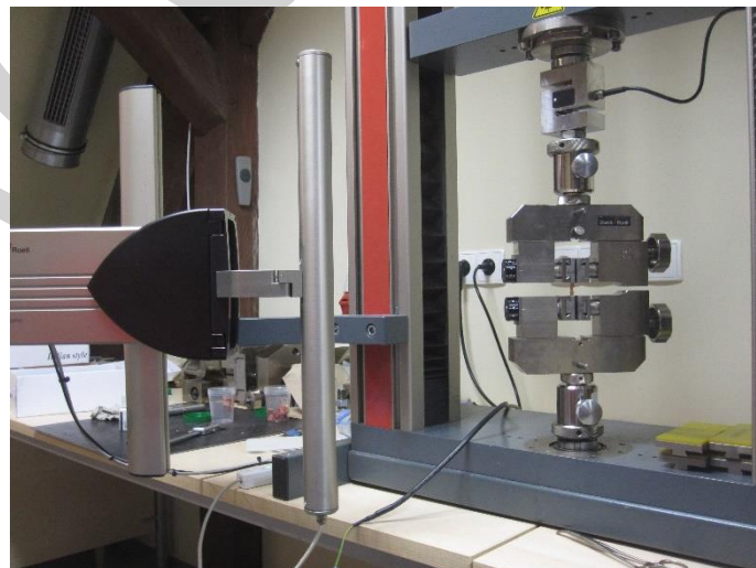
Fig. 1. Experimental stand with the video-extensometer.
