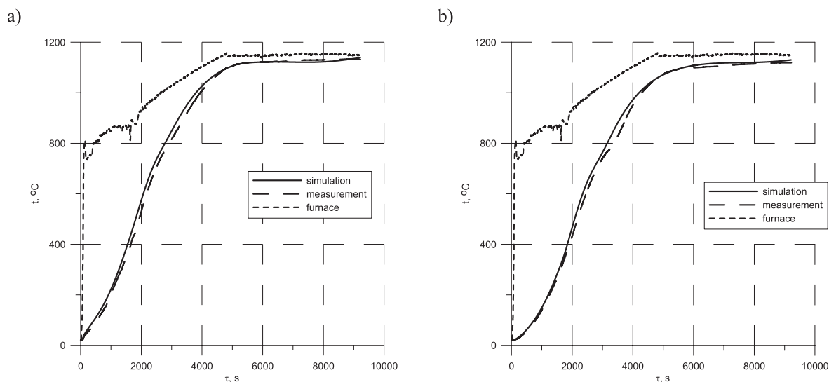
Fig. 4. The comparison of temperature distributions in the characteristic points: a) the top surface; b) the bottom surface
