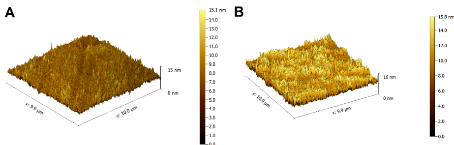
Fig. 8. AFM images of slide surface – non-modified (A), esterified with 1-decanol (B)
