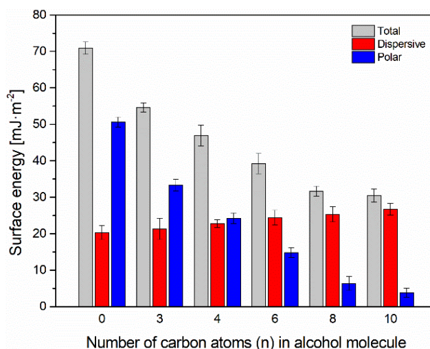
Fig. 10. Total surface energy and its components of glass surface – non-modified (n=0) and esterified (for 6 h) with the n=3-10 alcohols
