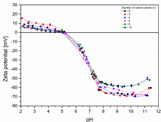
Fig. 11. pH dependence of zeta potential for non-modified and esterified glass surface for alcohols with different carbon chain length ( n )
