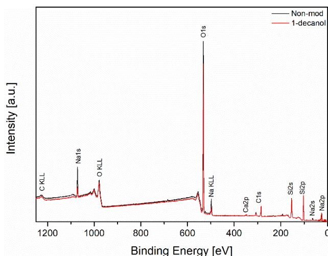
Fig. 2. XPS survey spectrum of glass surface before (non-modified) and after esterification with 1-decanol
