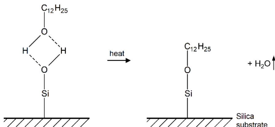
Fig. 1. Assumed mechanism of the esterification reaction after physisorption of the alcohol on the silica surface (Biggs and Grieser, 1994)
