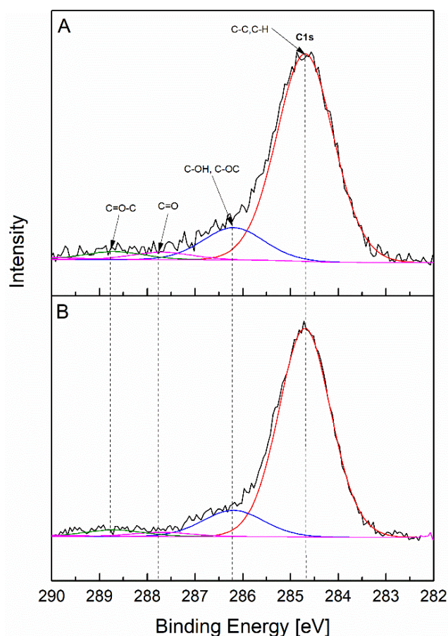
Fig. 3. High resolution XPS spectra and fitting curves of the C1s peak for glass before (A) and after (B) esterified esterification with 1-decanol
