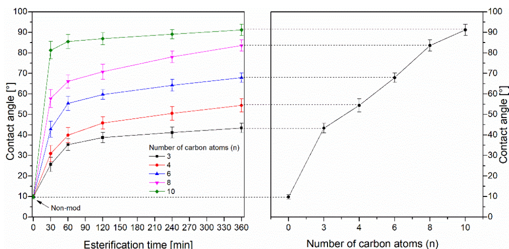
Fig. 9. Dependence of equilibrium water contact angles on the glass surface versus (A) esterification time for different chain lengths of alcohols, and (B) number of carbon atoms in alcohol chain after 6 h of esterification
