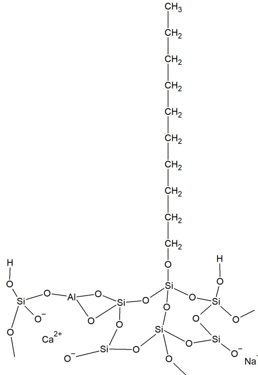
Fig. 6. Schematic representation of glass surface modification with 1-decanol
