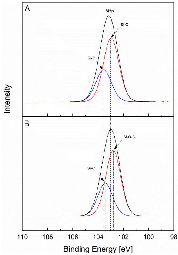
Fig. 4. High resolution XPS spectra and fitting curves of the Si2p peak for glass before (A) and after (B) esterified esterification with 1-decanol
