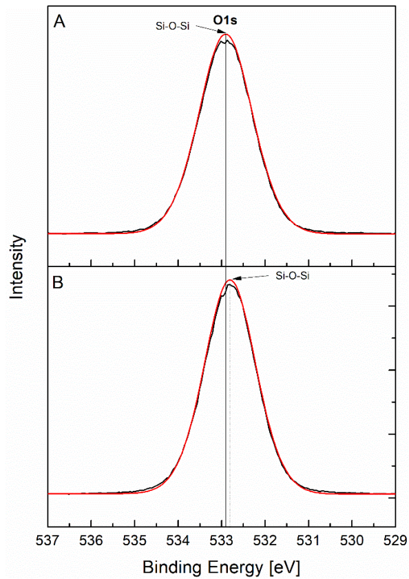
Fig. 5. High resolution XPS spectra and fitting curves of the O1s peak for glass before (A) and after (B) esterified esterification with 1-decanol
