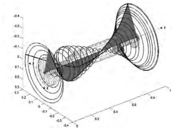
Fig. 13. Transverse rotor vibration at 358.8 Hz (damping 10.8%)
