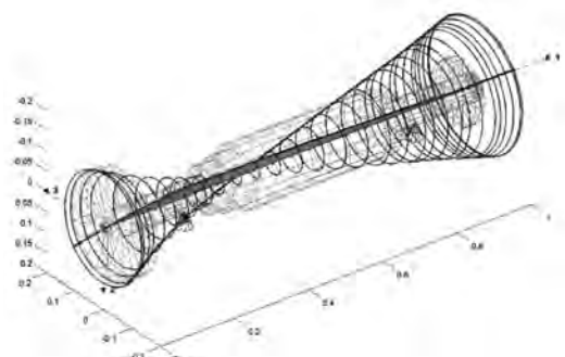
Fig. 11. Transverse rotor vibration at 157.6 Hz (damping 32.5%)
