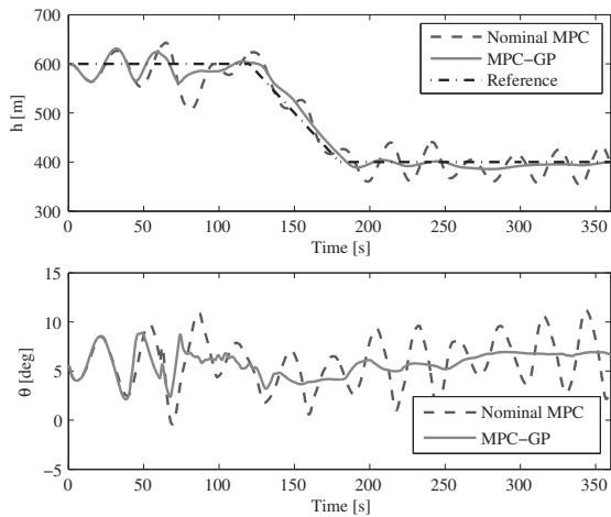
Fig. 12. Altitude and pitch angle responses in the 'stuck elevators' fault case, with comparison between nominal MPC and MPC with a GP model.
