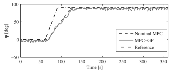
Fig. 14. Yaw angle response in the 'rudder runaway' fault case, with comparison between nominal MPC and MPC with a GP model.
