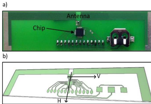
Fig. 3. A UHF RFID transponder with an omnidirectional antenna: a) sample #1; b) an HL3DEM antenna model.
