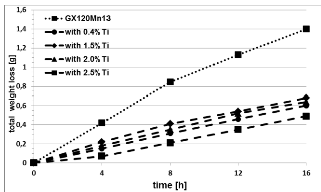
Fig. 5. Total weight losses of investigated cast materials steel after solution heat treated as a function of abrasion time
