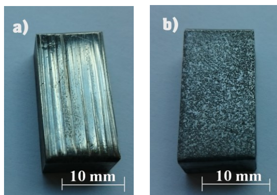
Fig. 6. Sample surface after abrasion test: cast Hadfield steel - a); tested cast steel with 2.0% Ti content - b)
