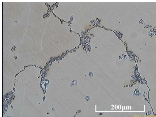
Fig. 1. As-cast microstructure of Hadfield steel; austenitic matrix with precipitates of alloyed cementite; nital etching [1]
