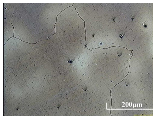
Fig. 3. Microstructure of cast Hadfield steel after solution heat treatment; austenitic matrix free from precipitates of alloyed cementite; nital etching [1]
