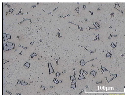
Fig. 4. Microstructure of cast steel (0.8% C, 16% Mn, 1.4% Cr, 2% Ti) after solution heat treatment; austenitic matrix with primary titanium carbides uniformly distributed in this matrix; nital etching [1]
