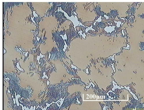
Fig. 2. As-cast microstructure of Hadfield steel with 1.4% Cr; austenitic matrix with numerous precipitates of alloyed cementite; nital etching [1]
