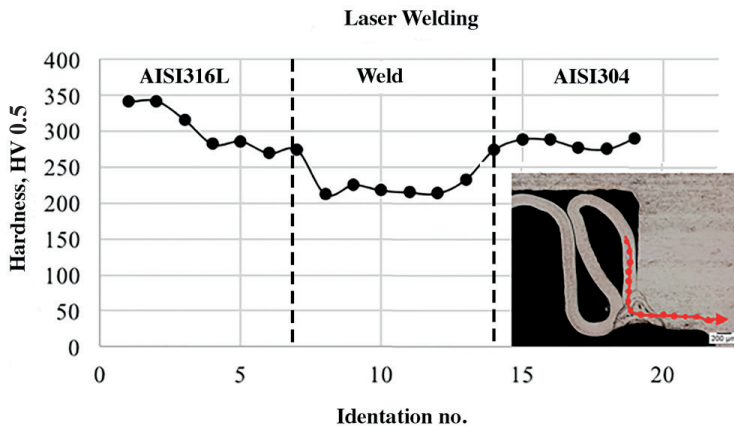
Fig. 5. Hardness profile on cross-section of laser-welded specimens
