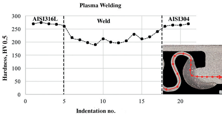
Fig. 6. Hardness profile on cross-section of microplasma-welded specimens
