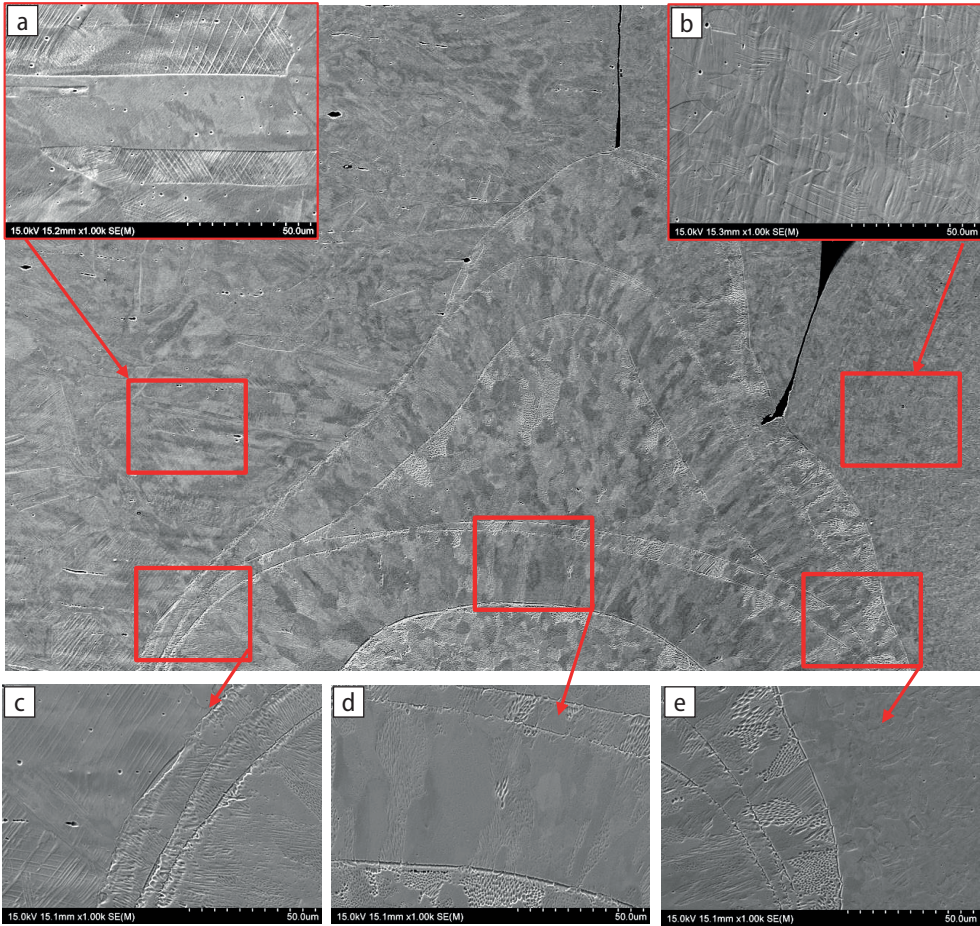
Fig. 3. Microstructure of laser beam welded joint: a) base material AISI 304; b) base material AISI 316L; c) microstructure of a weld-AISI 304; d) the microstructure of columnar grains; e) microstructure of a weld-AISI 316L
