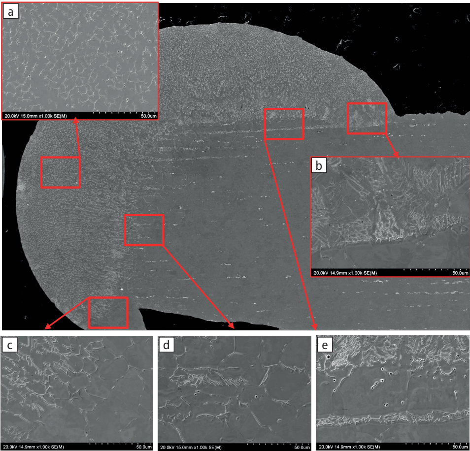
Fig. 4. Microstructure of microplasma-arc-welded joint: a) microstructure of central part the joint; c) microstructure of a weld-AISI 316L; (b, d, e) microstructure of a weld-AISI 304
