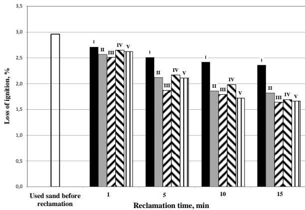
Fig. 9. Ignition loss values of the matrices reclaimed in the recycling process performed according to I-V methods
