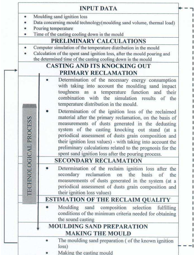
Fig. 2. Idea of the integrated recycling system of used moulding sands with organic resins
