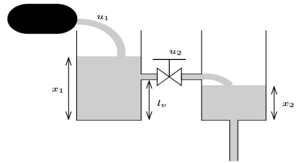
Fig. 3. Two-tank system.
