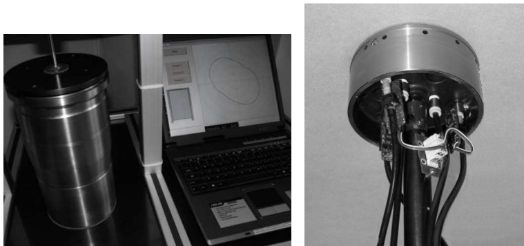
Fig. 13. A view of the Geoform device (left) and the gauging head (right).
