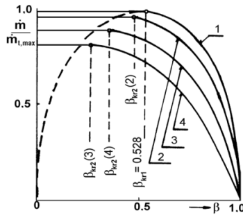
Fig. 3. The theoretical and actual mass flows as functions of the pressure ratio \beta .
