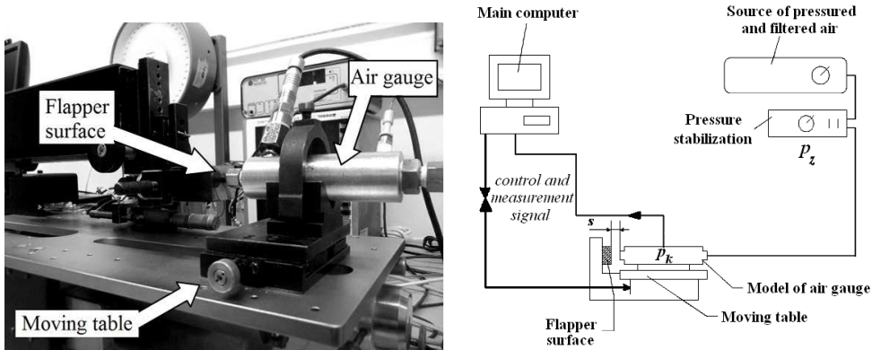
Fig. 10. A scheme of laboratory equipment for measurement of the air gauge static characteristics [19].
