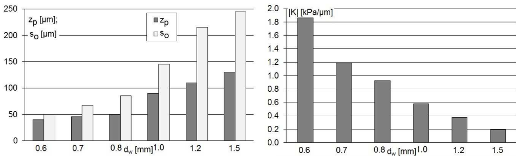
Fig. 9. The simulation results of measuring range z_p and its middle point s_0 (left) and multiplication (right).
