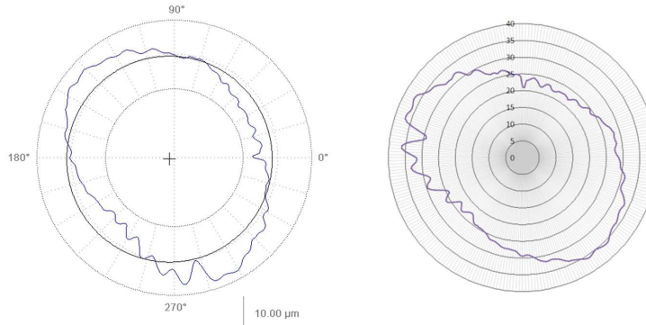
Fig. 16. The graphical representations of the same profile measured by the Talyrond 365 (left) and Geoform (right) devices.
