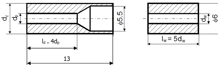
Fig. 11. The dimensions of chosen nozzles: measuring (left) and inlet (right).
