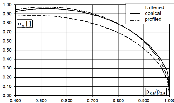
Fig. 2. The flow coefficient as a function of normalized values of the absolute back-pressure for different nozzles.
