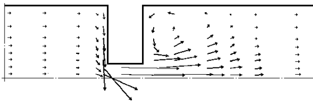
Fig. 6. The velocity vectors inside the air gauge measuring chamber [17].
