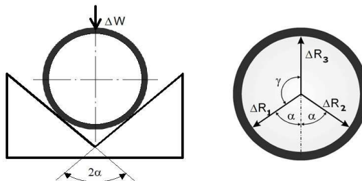
Fig. 15. The obtained results: \Delta R_1 , \Delta R_2 and \Delta R_3 , recalculated into the V-block measurement \Delta W .
