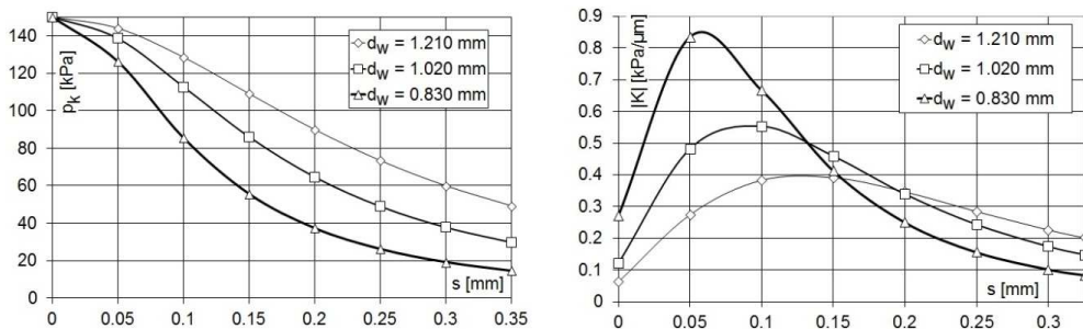
Fig. 8. The simulation results of static characteristics (left) and multiplication (right).
