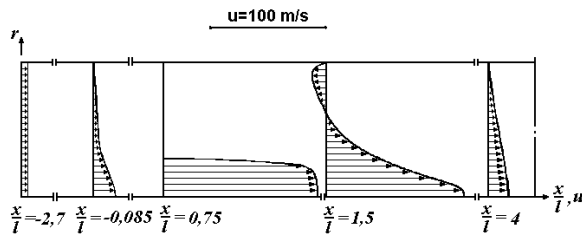
Fig. 5. The velocity profiles inside the air gauge measuring chamber [17].
