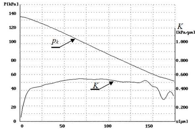
Fig. 12. The experimental static characteristics of a chosen air gauge.
