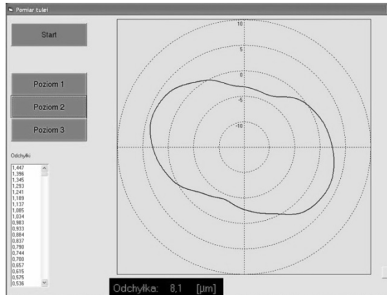
Fig. 14. An example of the measurement results presented on the screen [10].
