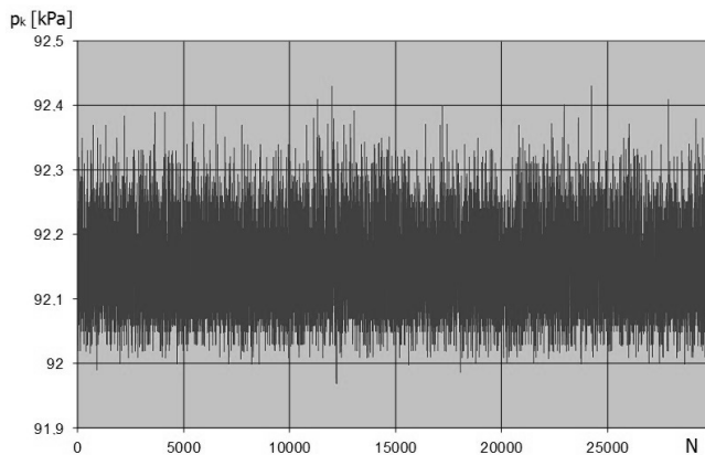
Fig. 7. The registered pressure fluctuations in the measuring chamber.
