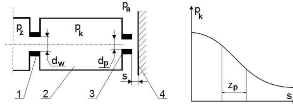
Fig. 1. An air gauge – its scheme (left) and static characteristics (right).
