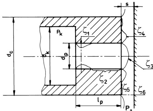
Fig. 4. The pressure losses in the flapper-nozzle area [10].
