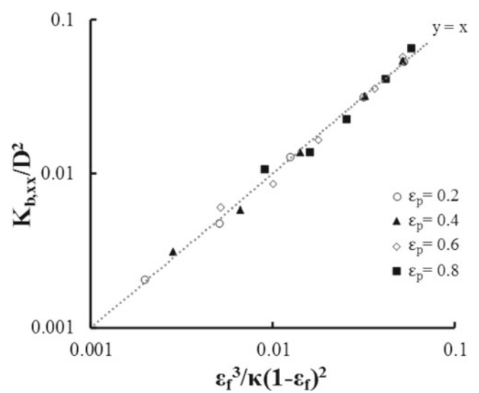
Figure 16. The comparison of suggested correlation in longitudinal direction with the obtained numerical permeability values
