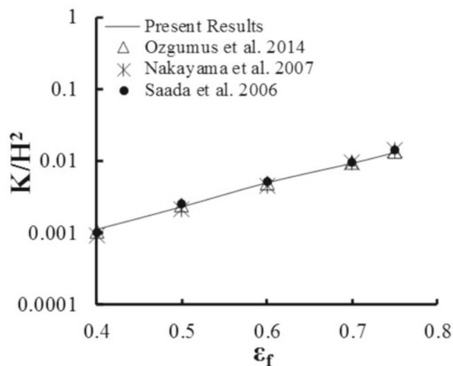
Figure 7. Comparison of permeability obtained in this study with the results reported in literature
