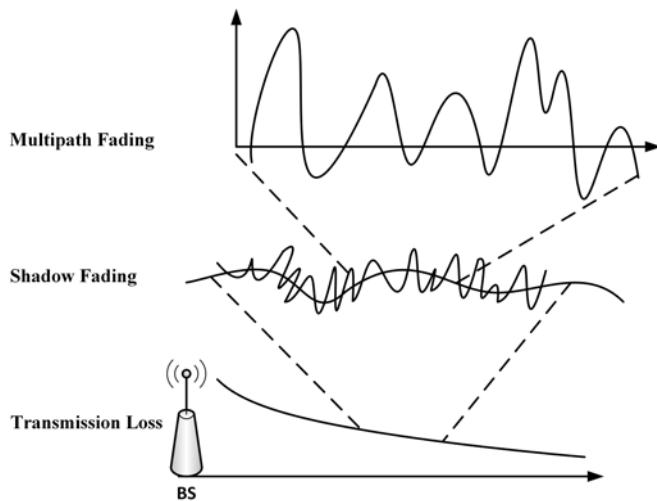
Fig. 2. Propagation loss in wireless channels
