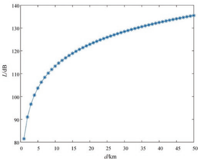
Fig. 3. The effect of d on the path loss
