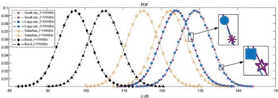
Fig. 6. The PDF curve of the path loss in each communication scenarios
