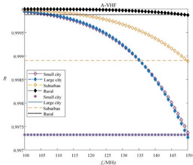
Fig. 10. The effect of the A-VHF's f_c on the reliability
