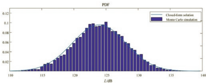
Fig. 5. The results of the Monte Carlo simulation compared with the closed-form solution
