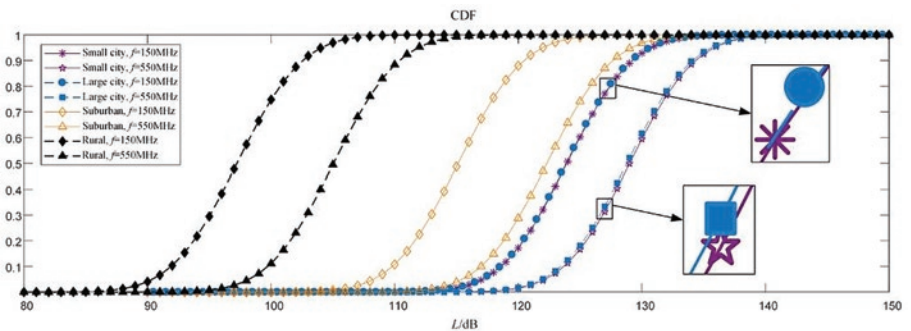
Fig. 7. The CDF curve of the path loss in each communication scenarios
