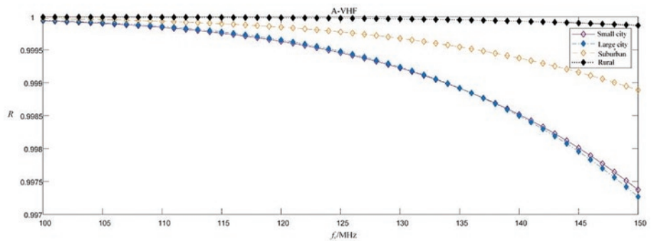
Fig. 8. The effect of the A-VHF's f_c on the reliability
