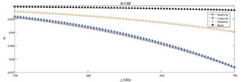
Fig. 9. The effect of the B-UHF's f_c on the reliability
