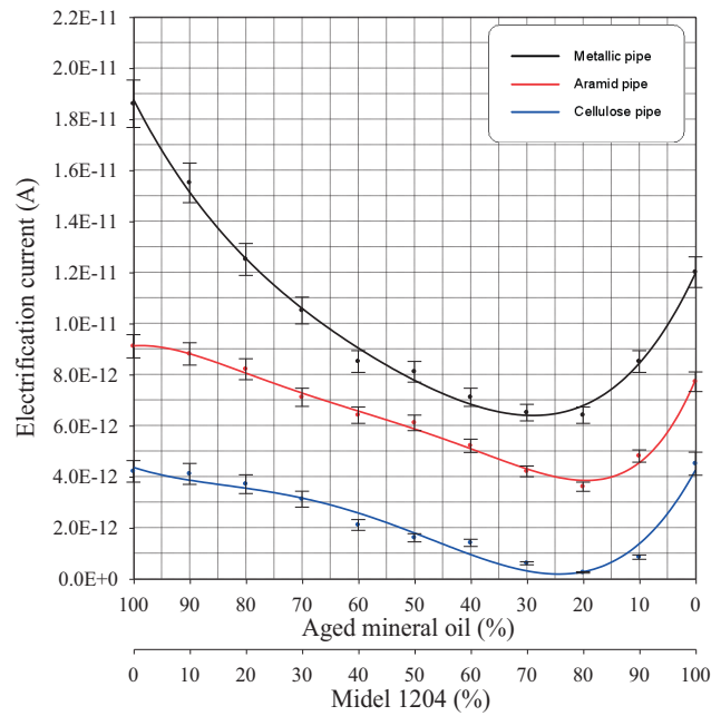
Fig. 7. Electrification current vs. percent content of natural ester Midel 1204 and aged mineral oil in the mixtures
