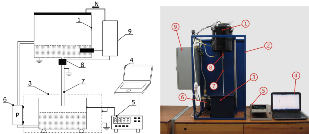
Fig. 1. Layout of the test stand with a flow pipe for testing streaming electrification of insulating fluids: 1 – top tank, 2 – supporting structure, 3 – Faraday cage with measuring tank located inside, 4 – measuring computer, 5 – electrometer, 6 – pump, 7 – measuring pipe, 8 – solenoid valve, 9 – control box
