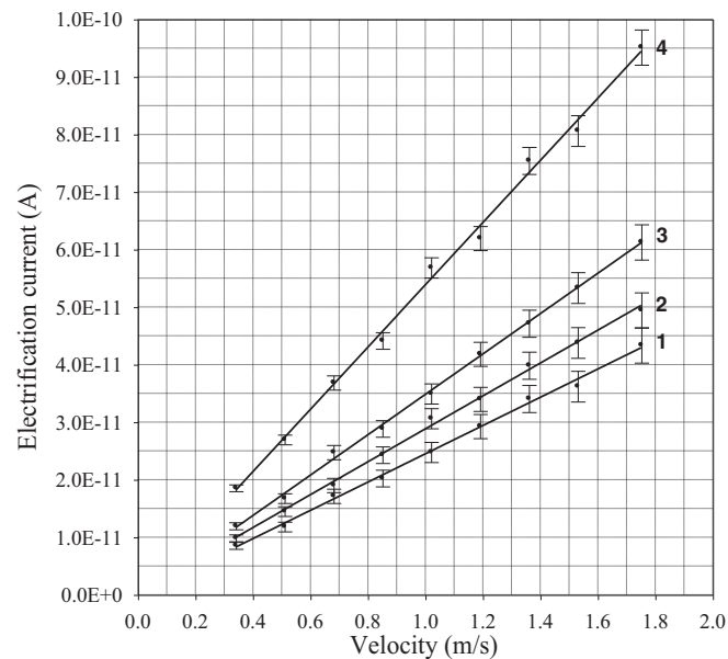
Fig. 2. Electrification current of insulating liquids vs. flow velocity through a metallic pipe: 1 – fresh mineral oil, 2 – synthetic Midel 7131, 3 – natural Midel 1204, 4 – aged mineral oil
