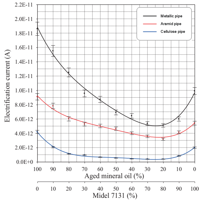
Fig. 6. Electrification current vs. percent content of synthetic ester Midel 7131 and aged mineral oil in the mixtures
