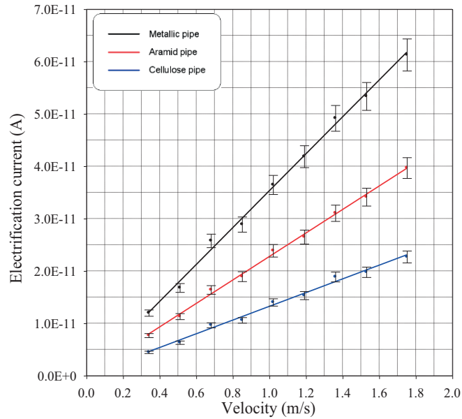
Fig. 3. Electrification current vs. flow velocity of natural ester Midel 1204 through the pipes made of various materials
