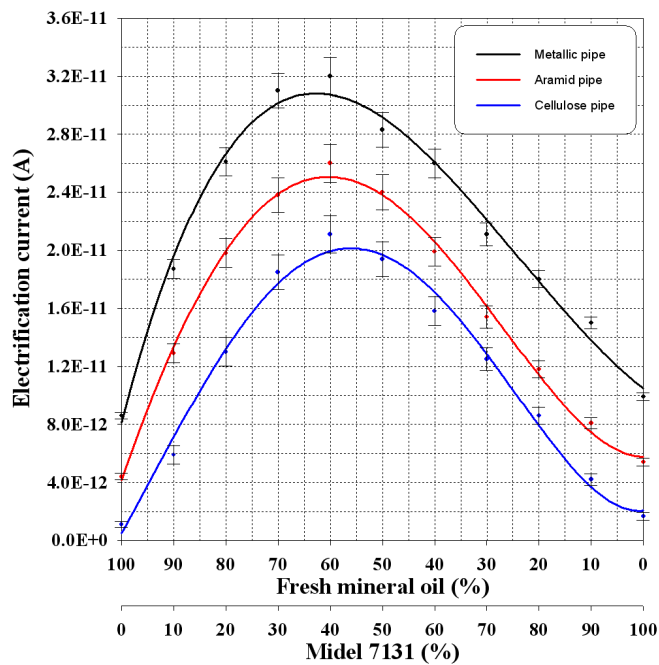
Fig. 4. Electrification current vs. percent content of synthetic ester Midel 7131 and fresh mineral oil in the mixtures
