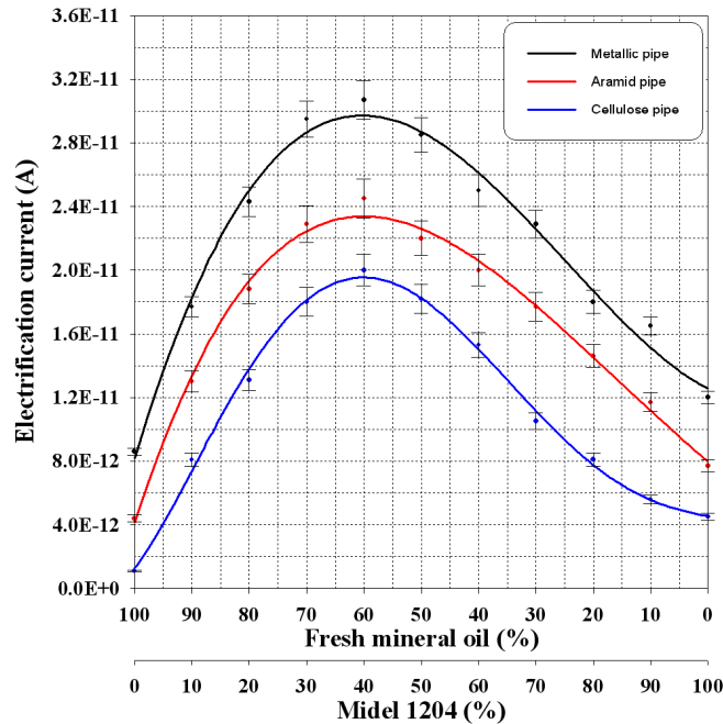
Fig. 5. Electrification current vs. percent content of natural ester Midel 1204 and fresh mineral oil in the mixtures
