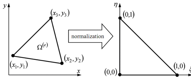
Fig. 2. Normalization of the triangular finite element
