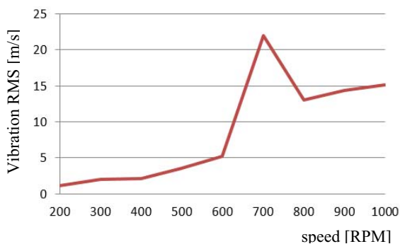
Fig. 7. Dependence of the speed on vibration values of the mechanical systems using shaft couplings Hardy GJ9
