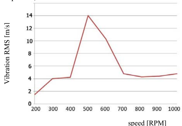
Fig. 5. Dependence of the speed on the vibration values of mechanical system using pneumatic coupling pressurized on the pressure value 100 kPa
