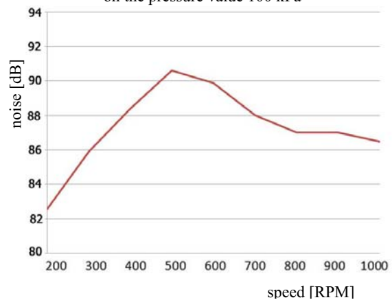
Fig. 6. Dependence of the speed on the noise level of the mechanical system using pneumatic coupling pressurized on the pressure value 100 kPa
