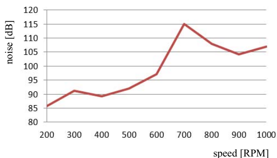
Fig. 8. Dependence of the speed on the noise level in the mechanical system using shaft couplings Hardy GJ9
