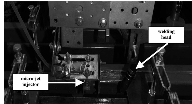
Fig. 1. Montage of welding head and micro-jet injector
