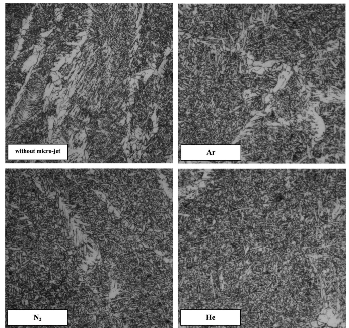
Fig. 3. Acicular ferrite in weld (68-73%) in terms on micro-jet gases, magnification ×200
