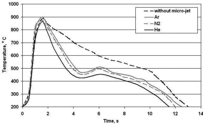
Fig. 2. Weld cooling conditions (without micro-jet and with different cooling gases)
