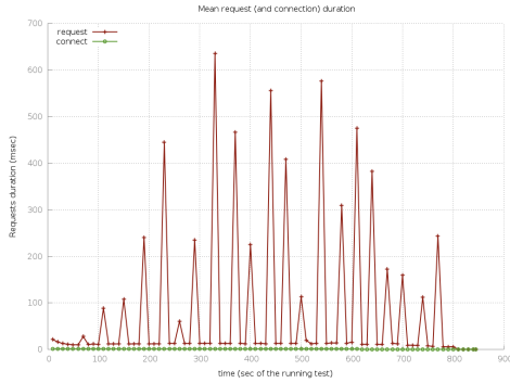
Figure 7. Mean time of saving data document to the database during the second test.
