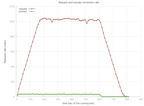
Figure 4. Data submission rate during the 1st test.
