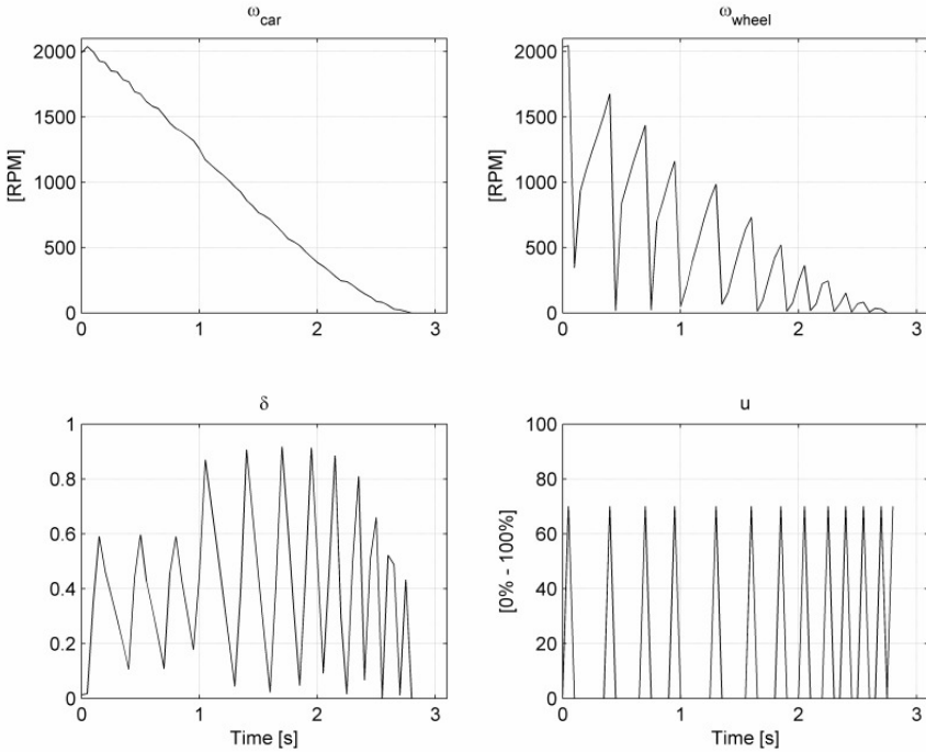
Fig. 7. Braking experiment.
