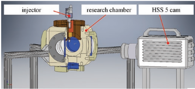
Fig. 1. Test bench
