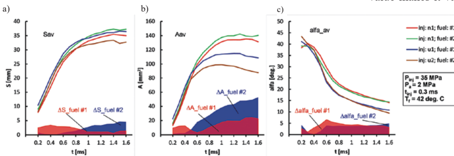
Fig. 6. Evaluation of average fuel spray indicators with limit values and value ranges: a) stream range – S, b) stream surface area – A, c) stream cone angle – alpha
