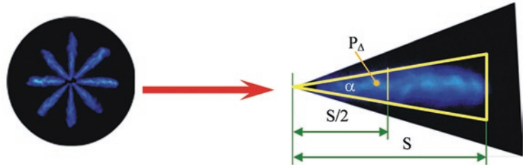
Fig. 2. Method for determining the fuel stream cone angle
