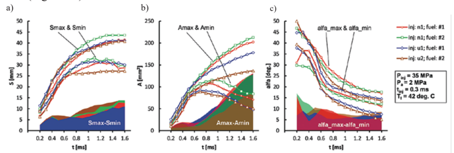
Fig. 5. Evaluation of limit values and differences of these values during fuel injection: a) stream range – S , b) stream surface area – A , c) stream cone angle – \alpha
