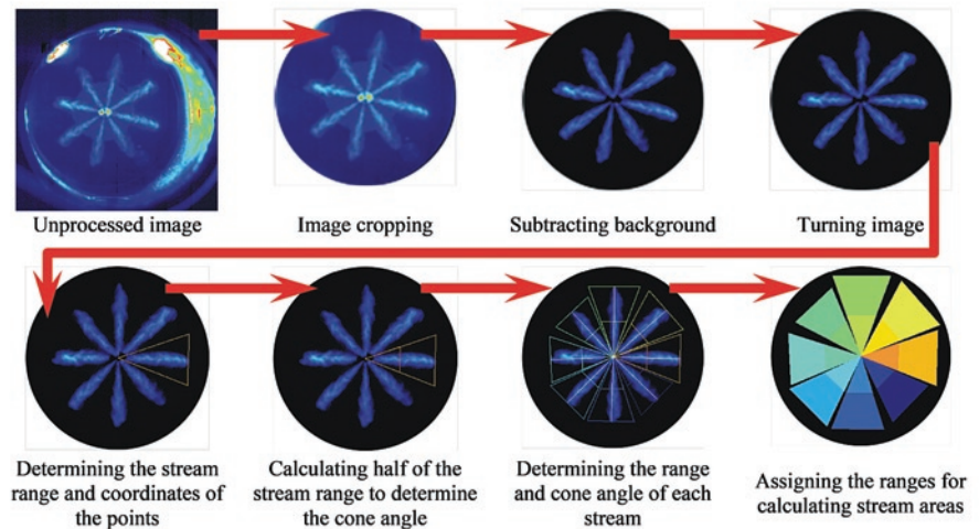
Fig. 3. Image processing and determining the geometric indicators of the fuel stream
