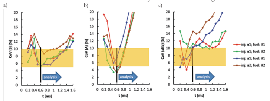
Fig. 6. Evaluation of average fuel spray indicators with limit values and value ranges: a) stream range – S, b) stream surface area – A, c) stream cone angle – alpha
