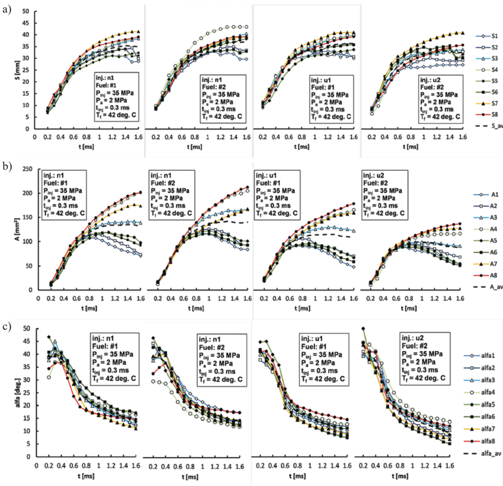
Fig. 4. Results of fuel spray indicator tests: a) fuel stream range – S , b) fuel stream area – A , c) stream cone angle – \alpha
