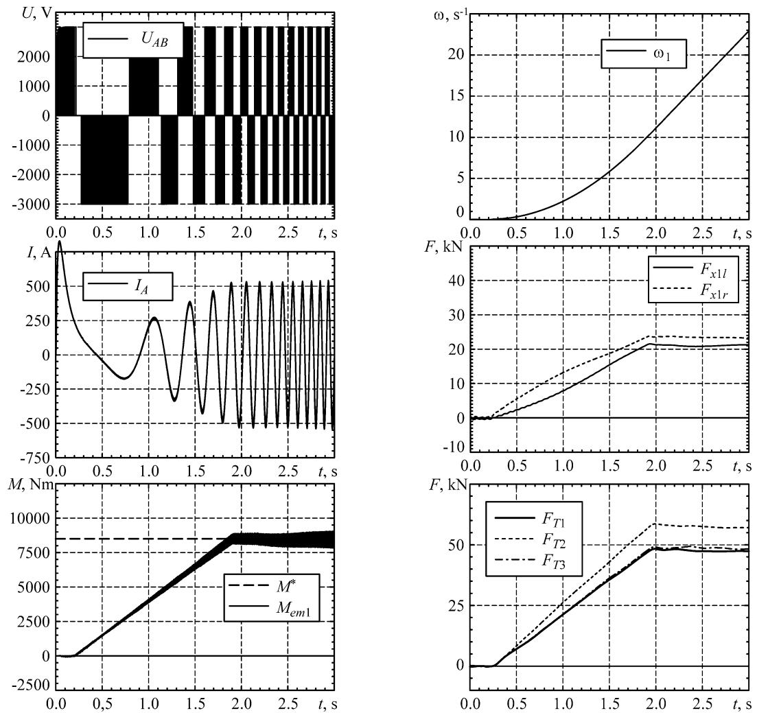
Fig. 1. Electromechanical processes at start and acceleration
