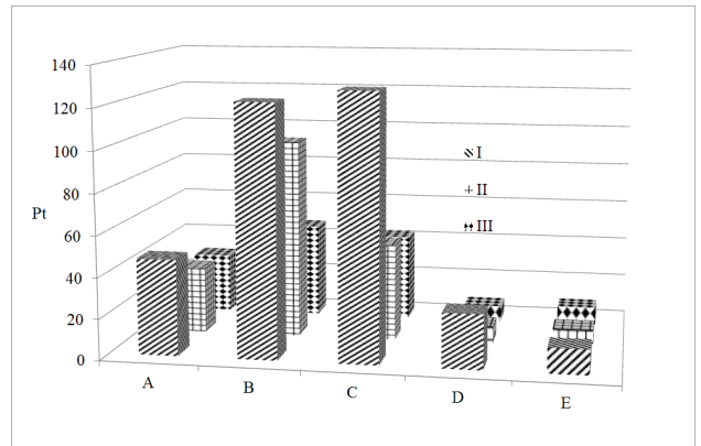
Fig. 3. Results of LCA analysis in the form of a histogram. Source: Central Statistical Office, functional unit 1000 PLN of products [11];
