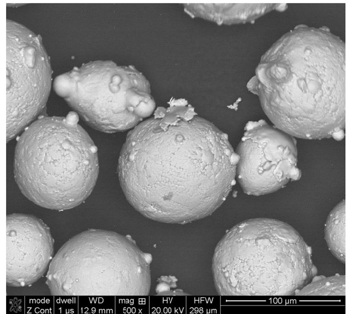
Fig. 10. Not completed birth of some droplets from particles; the jammed droplets subjected to rapid solidification in the contact with water; the droplets remaining inside the mother-particle subjected to slow solidification
