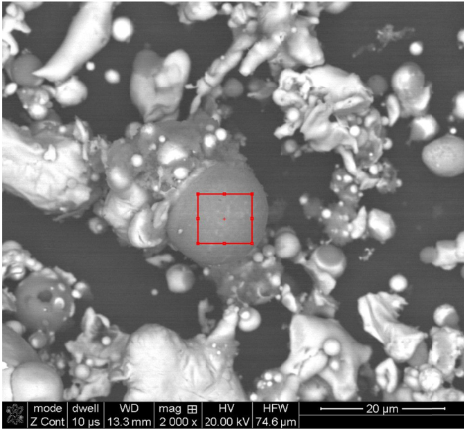
Fig. 4. Al-enriched core (droplet) released from the mother Fe-40Al particle
