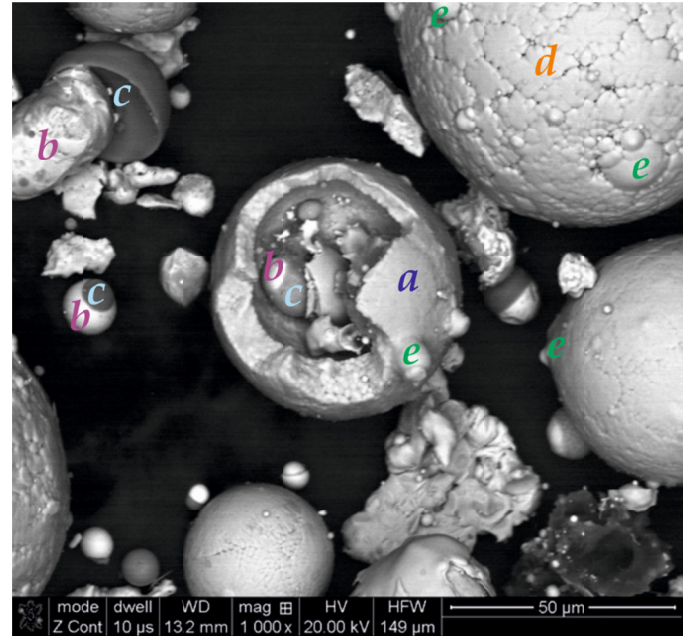
Fig. 6. Crushed particle, (a); the solid shell of the damaged particle with a varying thickness which results from a chaotic rotation of this particle and resultant unevenly occurring solidification during the particle motion through air / gas; axial segregation (separation into iron rich part, (b), and aluminum rich part, (c), due to the one-axial revolution of a given droplet); a cellular (honey-comb) structure of the particle shell, (d); some protruding droplets, partially born / jammed in the solid shell of the particle, (e)
