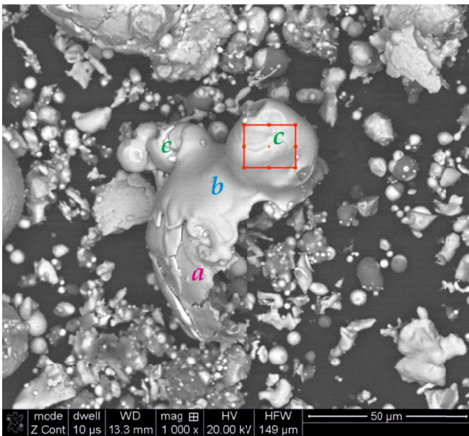
Fig. 5. Birth of some droplets, (c), from the Fe-40Al particle partially damaged, (a), due to the stroke of an accidental droplet, (b) and settlement onto the water surface
