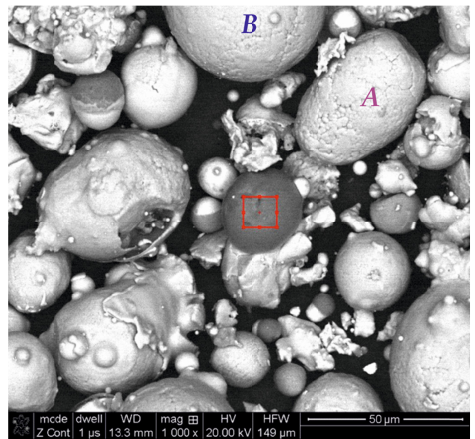
Fig. 7. Aluminum enriched part of a doublet visible in the image center (with the marked window / area for the measurement of the elements concentration)
