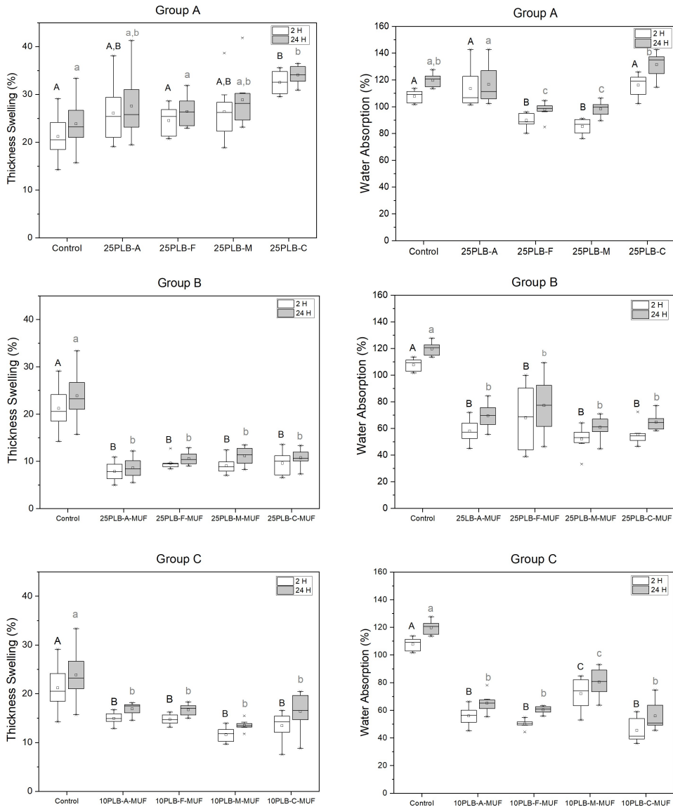
Fig. 2. Thickness swelling and water absorption (2 and 24 h) of particleboards made with partially liquefied bark of different sizes. Error bars represent standard deviations. Values labelled with different letters are statistically different at p < 0.05 (ANOVA and Tukey test)
