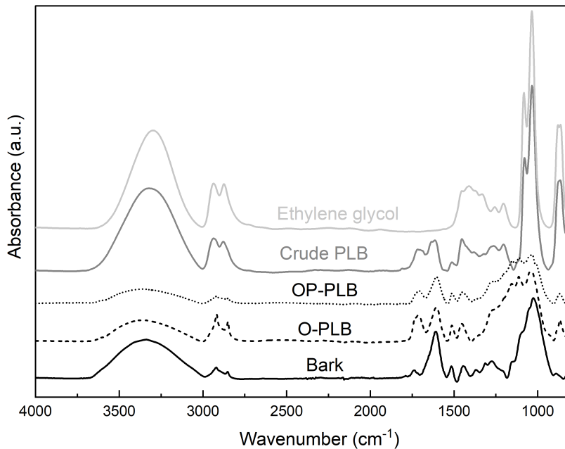
Fig. 1. Fourier transform infrared (FTIR) spectra of raw bark, crude partially liquefied bark (PLB), oven-dried PLB (O-PLB), oven-dried purified PLB (OP-PLB), and ethylene glycol
