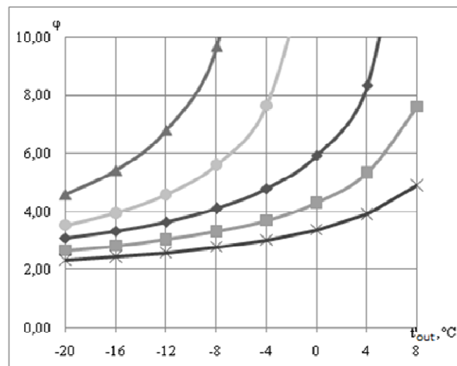
Fig. 2. Dependence of the conversion factor on the outside air temperature with different ratios of energy carriers in the ground and surface heat exchangers with a characteristic component of heat for heating and ventilation processes ( own study ):
