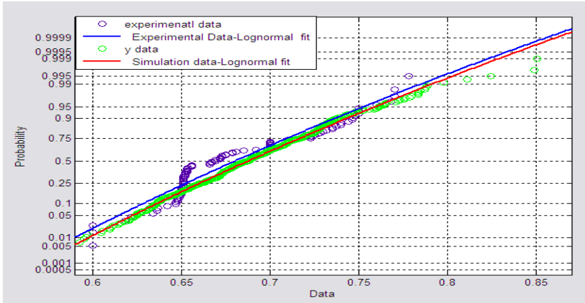
Fig. 3. Log Normal Probability Paper Plot for R_7^*
