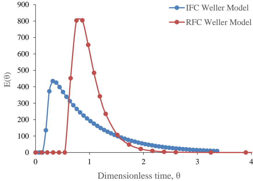
Fig. 5. Presentation of dimension-less RTD data experimentally measured (dots) and modeled (continuous lines) via the Weller model for a V-030 (IFC cell) and RFC-100
