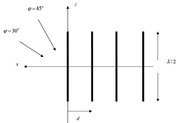
Fig. 2. The DOA estimation with a 4-dipole antenna array, separation ( \varphi_1 = 30^\circ and \varphi_2 = 45^\circ , and \theta = 90^\circ )
