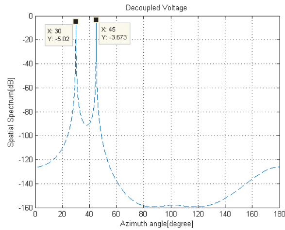
Fig. 4. The DOA of incoming signals to array from \varphi_1 = 30^\circ and \varphi_2 = 45^\circ and \theta = 90^\circ in the presence of mutual coupling with compensation
