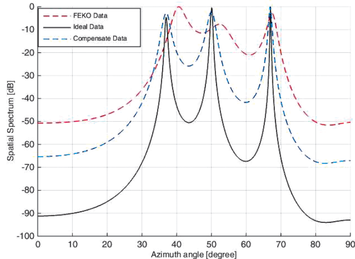
Fig. 6. The DOA estimation of incoming signals to array from \varphi_1 = 37^\circ and \varphi_2 = 50^\circ , and \varphi_3 = 67^\circ for different types of voltages as input in the MUSIC algorithm
