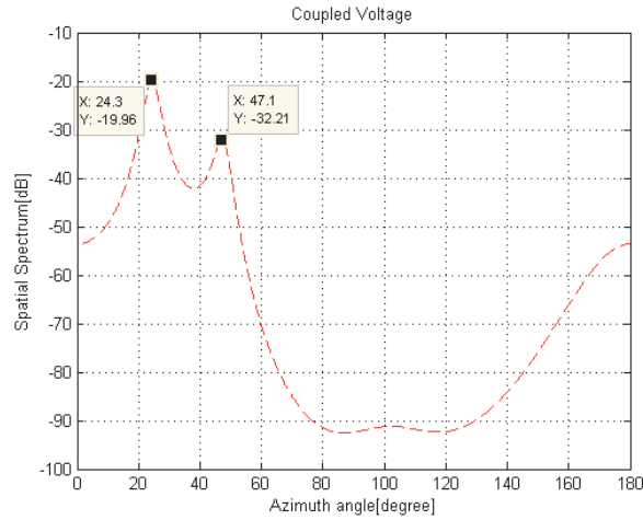
Fig. 3. The DOA of incoming signals to array from \varphi_1 = 30^\circ and \varphi_2 = 45^\circ and \theta = 90^\circ in the presence of mutual coupling without compensation
