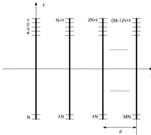
Fig. 1. Illustration of dipole antennas array
