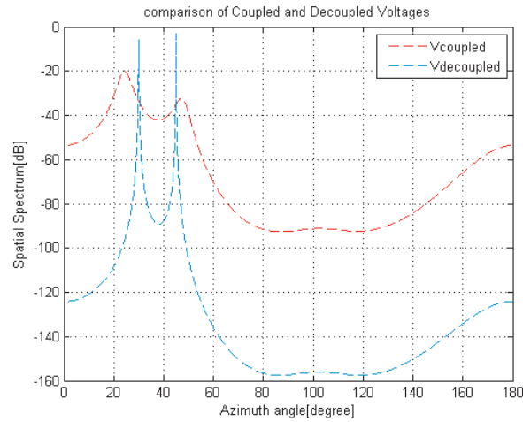
Fig. 5. The DOA estimation of incoming signals to array from \varphi_1 = 30^\circ and \varphi_2 = 45^\circ , and \theta = 90^\circ in the presence of mutual coupling with compensation and without compensation
