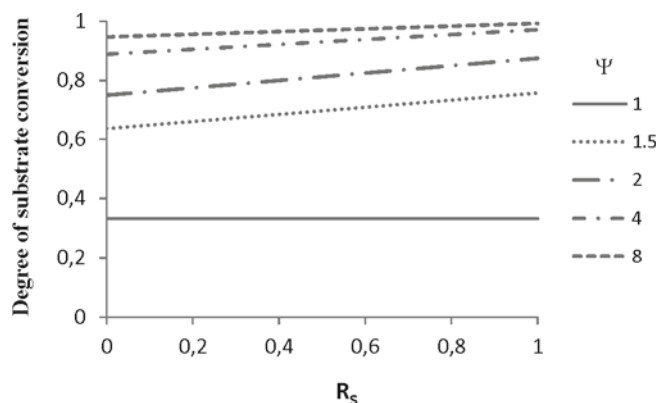
Figure 4. The simultaneous effect of the value of R_S and \Psi on the degree of substrate conversion (based on Equation (15))
