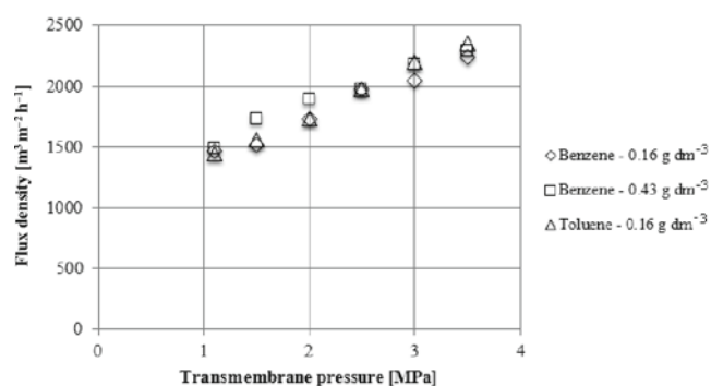
Figure 7. The effects of pressure and the concentrations of benzene and toluene at the process temperature of 24^\circ\text{C} on the permeate flux (AFC 90 reverse osmosis membrane)
