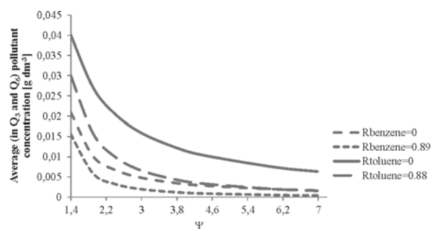
Figure 9. Average pollutant concentration in the merged outgoing (Q 3 and Q 6 ) streams as a function of \Psi and R_s (based on Equation (14))
