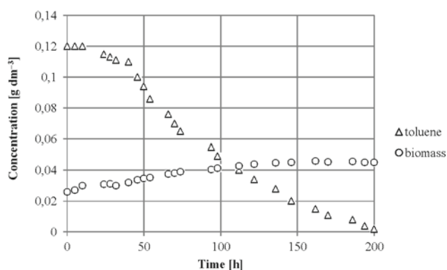
Figure 6. Batch process of toluene removal ( c_{s,0} = 0.12 \text{ g dm}^{-3} , 24^\circ\text{C} ): ( \Delta ) toluene concentration, ( \circ ) biomass concentration
