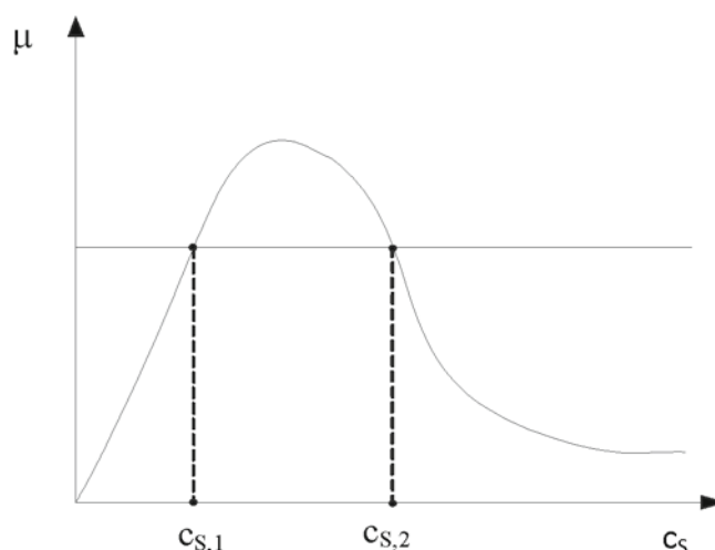
Figure 2. Steady states in the case of microbial kinetics with a substrate inhibition (one value of \mu corresponds to two states i.e. two different biomass concentration and two different c_{S,2} )
