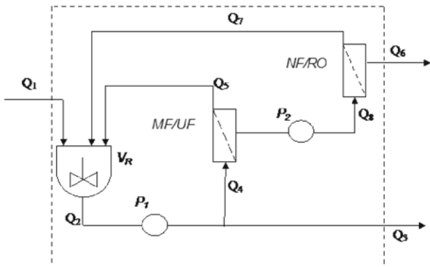
Figure 3. Schematic diagram of a bioreactor with two separation modules (VR – reactor volume, MF/UF – first step of filtration, NF/RO – second step of separation)
