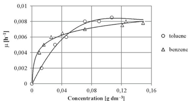
Figure 5. Kinetics (24°C) of benzene ( \Delta ) and toluene ( \circ ) biodegradation by P. fluorescens strain (PCM 2123)
