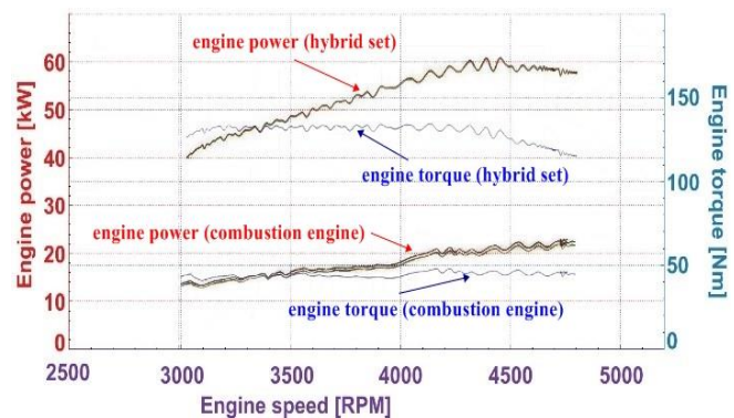
Fig. 12. Course of power and torque of the internal combustion engine and hybrid drive: torque [Nm], useful power [kW]
