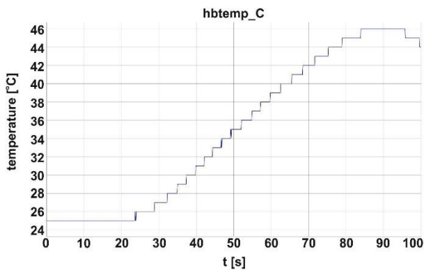
Fig. 18. The course of the inverter temperature at the time of electric motor operation
