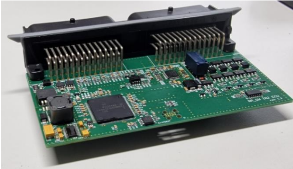
Fig. 9. Injection ECU – PCB view
