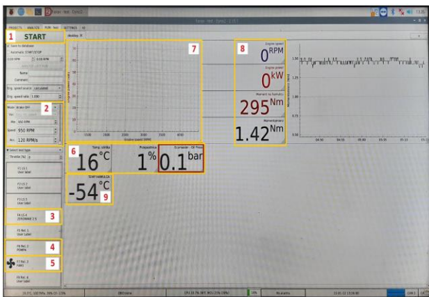
Fig. 2. Performance parameters of the hybrid set analyzed on the test stand: 1 – measurement start button, 2 – measurement mode selection, 3 – torque sensor setting to zero, 4 – water pump start button, 5 – cooling tower fan start button, 6 – ICE working parameters (temperature, throttle opening, oil pressure), 7 – characteristics chart, 8 – brake and torque sensor operating parameters, 9 – brake coolant temperature
