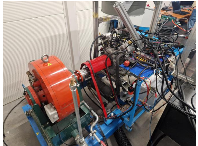
Fig. 4. View of the engine brake and drive set
