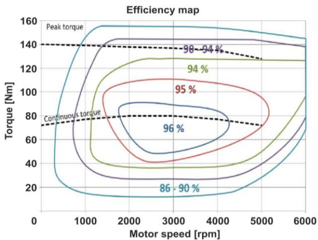
Fig. 8. Torque and speed motor characteristics – EMRAX 208
