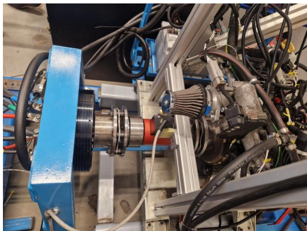
Fig. 5. View of a used electric motor and its connection
