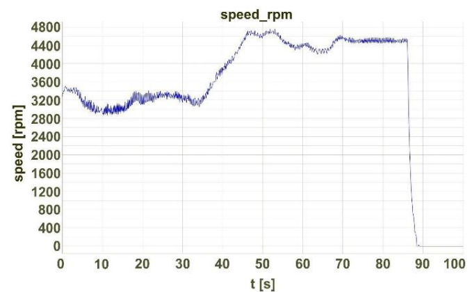
Fig. 17. The rotational speed of the electric motor for given operating conditions
