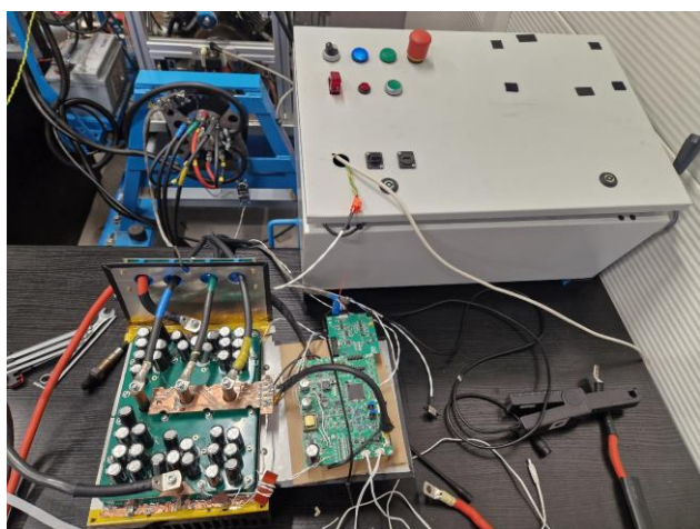
Fig. 6. Control and measurement system assembly – hybrid assembly dynamometer
