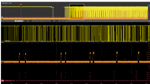
Fig. 10. An example of a sequence of injection pulses. The first two pulses after the rotational speed occur are caused by fuel injection and facilitating engine start-up.
