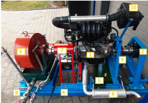
Fig. 1. View of the stand in a hybrid combination with a 4-cylinder in-line engine: 1 – 4-cylinder IC engine, 2 – EMRAX electric motor, 3 – water-cooled Eddy current brake, 4 – test stand main frame, 5 – engine oil tank, 6 – exhaust system, 7 – drive shaft between ICE and brake, 8 – cooling system connections, 9 – drive shaft between ICE and EMRAX with torque sensor, 10 – ICE intake air filter
