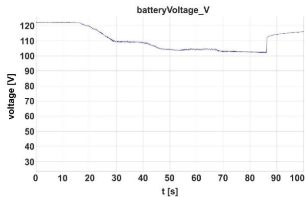
Fig. 14. Voltage drop on the battery cells of the hybrid set
