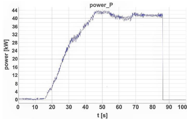
Fig. 13. Change of electric motor power in series connection with medium propeller load
