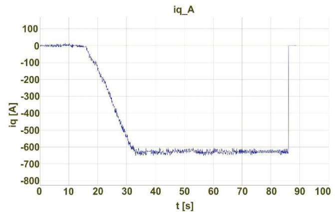
Fig. 16. Change of the current value in the electric motor
