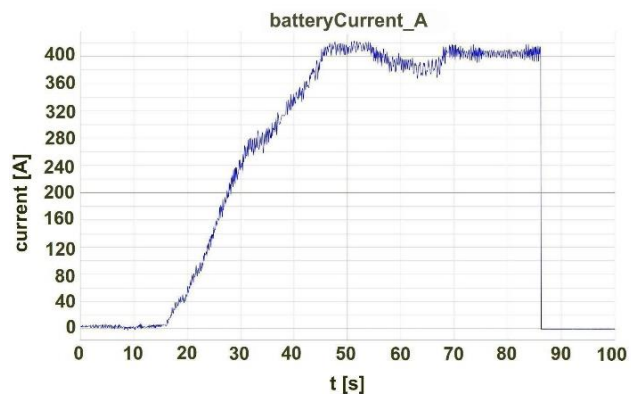
Fig. 15. Change of the current in the battery cells during the period of increasing the power of the electric motor
