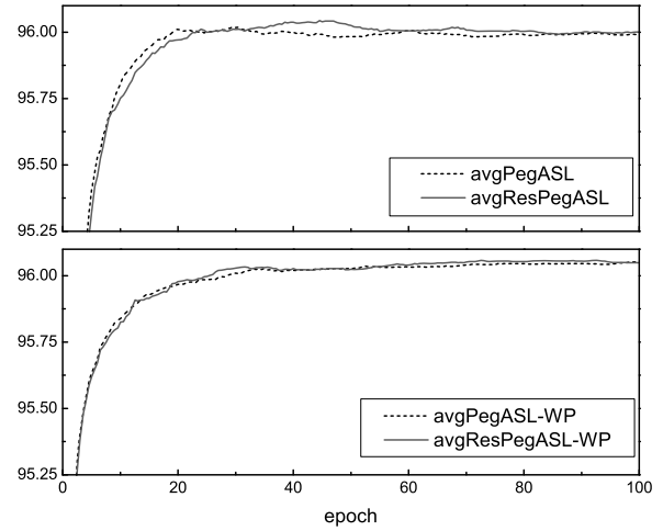
Fig. 1. Results in terms of the F-measure through epochs for the restricted and non-restricted version of the Pegasos algorithm with the averaged sum loss on shallow parsing. The curves are drawn with k = 10 .
