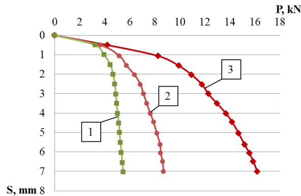
Fig. 5. Graph "Loading– Settlement" 1st stage of test for three different sizes of plate segments: 1 – 75 mm; 2 – 125 mm; 3 – 175 mm
