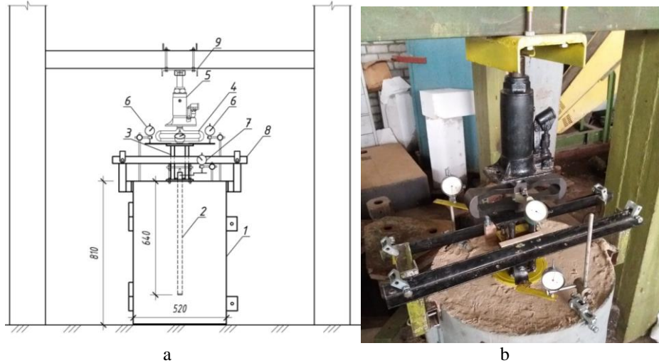
Fig. 1. Test facility: a – test facility layout: 1 – cylinder-shaped tank; 2 – pile model; 3 – plate segment model; 4 – mechanical load gauge; 5 – hydraulic jack; 6 – deflectometer (to identify plate settlement); 7 – indicators (to identify pile settlement); 8 – racks for balanced plate settlement; 9 – fixing jack support (12 mm plate); b – photo
