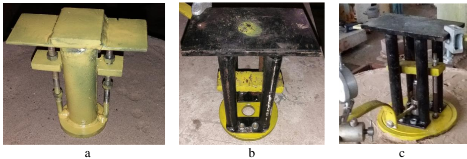
Fig. 3. The photo of plate model segments depending on pile diameter ( d ) and conditional distance between piles: a – 3d , (75 mm); b – 5d , (125 mm); c – 7d (175 mm)
