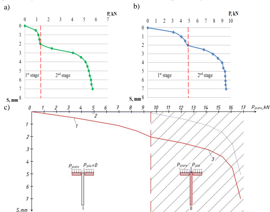
Fig. 6. Graph "Loading– Settlement". II nd test of plate segments: 75 mm (a), 125 mm (b), 175 mm (c); 1 – plate settlement, 2 – pile settlement due to additional loading; 3 – settlement of plate joining a pile
