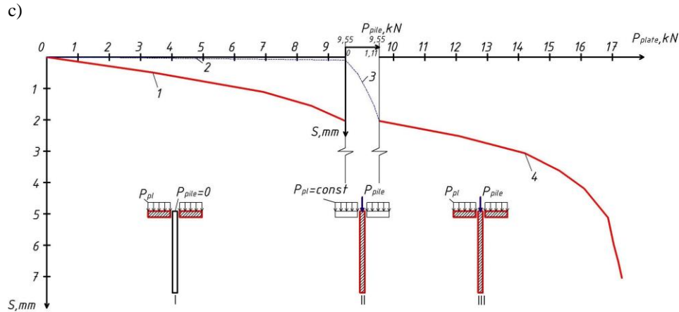
Fig. 7. Graph "Loading- Settlement". III rd test of plate segments: 75 mm (a), 125 mm (b), 175 mm (c); 1 – 1 st stage of plate settlement, 2 – 1 st stage of pile settlement; 3 – 2 nd stage of pile loading; 4 – settlement of plate joining a pile
