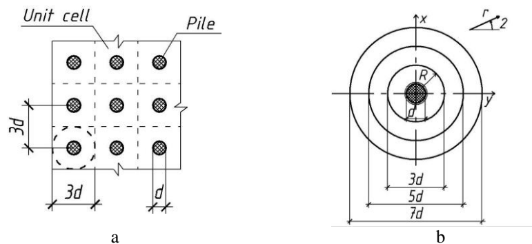
Fig. 2. Soil body with regularly placed piles and unit cell model (a) plate segment constructions (b): d – pile diameter, 3d , 5d i 7d – unit cell size (distance between piles) R – unit cell radius
