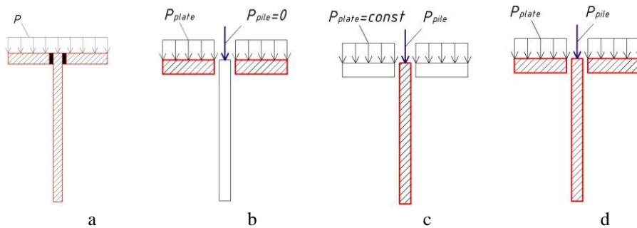
Fig. 4. Layout of load combinations of pile foundation elements: a – 1 st test; b – 1 st stage of II nd and III rd tests; c – 2 nd stage of III rd test; d – 2 nd stage of II nd test and 3 rd stage of III rd test
