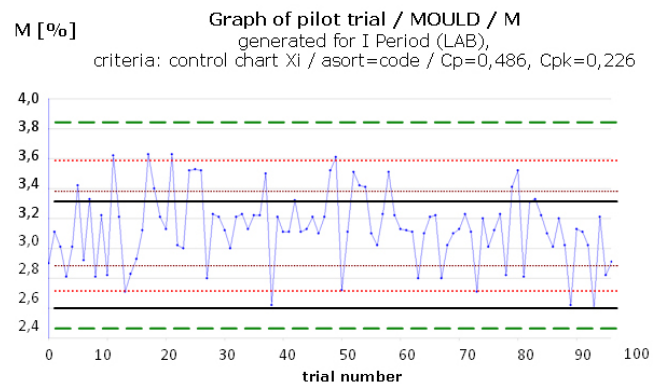
Fig. 3. Control chart for moisture – I period (continuous lines – tolerance limits, dashed and dotted lines – control and warning limits, respectively, on levels 2\sigma and 1\sigma )
