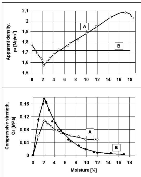
Fig. 1. Influence of moisture on compressive strength of a green sand, A – for continuous work of compacting the sample, B – for constant apparent density, \rho_0=1,715 \text{ [Mg/m}^3\text{]} (prepared on the basis of [1])
