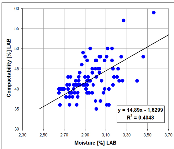
Fig. 7. Matching of results of moisture and compactability measurements obtained in the laboratory
