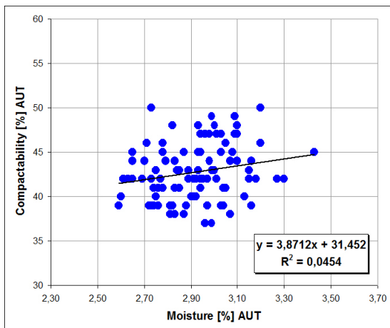
Fig. 8. Matching of results of moisture and compactability measurements obtained automatically
