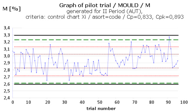
Fig. 4. Control chart for moisture – II period (interpretation of limits as in Fig.3)
