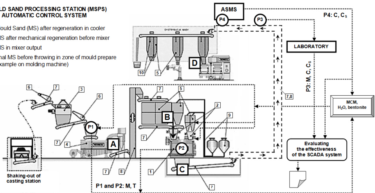
Fig. 2. Sand processing plant with automated quality control system, where: 1. Turbine mixer MTI, 2. Set of extensometric scales, 3. Sand screen, 4. Fluidizing cooler, 5. Containers of sand and additives, 6. Electromagnetic separator, 7. Belt conveyors, 8. Elevator, 9. Pneumatic transport, 10. Probes of upper and lower level, ASMS – Automated Sand Measurement System, MCM – Main Control Module (lot of water and bentonite), P1, P2, P3, P4 – Measuring points, M – Moisture, T – Temperature, C – Compactability, C_s – Compressive strength (own work on the basis of www.technical.com.pl )
