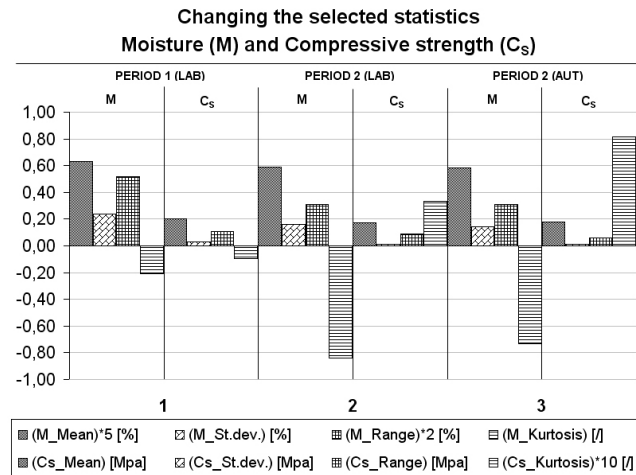
Fig. 5. Selected quantitative descriptive statistics for the two compared periods of work of the sand processing station
