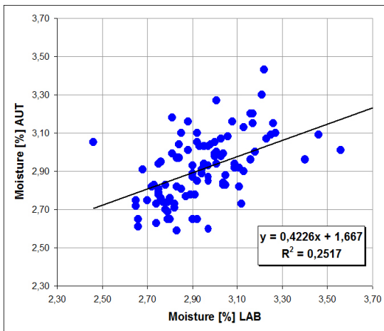
Fig. 6. Matching of results of moisture measurements obtained in the laboratory and automatically
